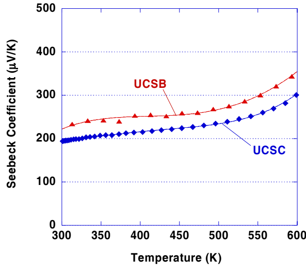
Figure 1. Seebeck coefficients of (\text{InGaAs})_{0.8}(\text{InAlAs})_{0.2} with 0.3% ErAs nanoparticles vs temperatures from 300 K to 600 K. The measurements were separately carried out at UCSB and UCSC.
