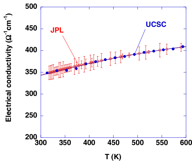
Figure 2. Electrical conductivity of (\text{InGaAs})_{0.8}(\text{InAlAs})_{0.2} with 0.3% ErAs nanoparticles measured at UCSC and JPL, respectively.
