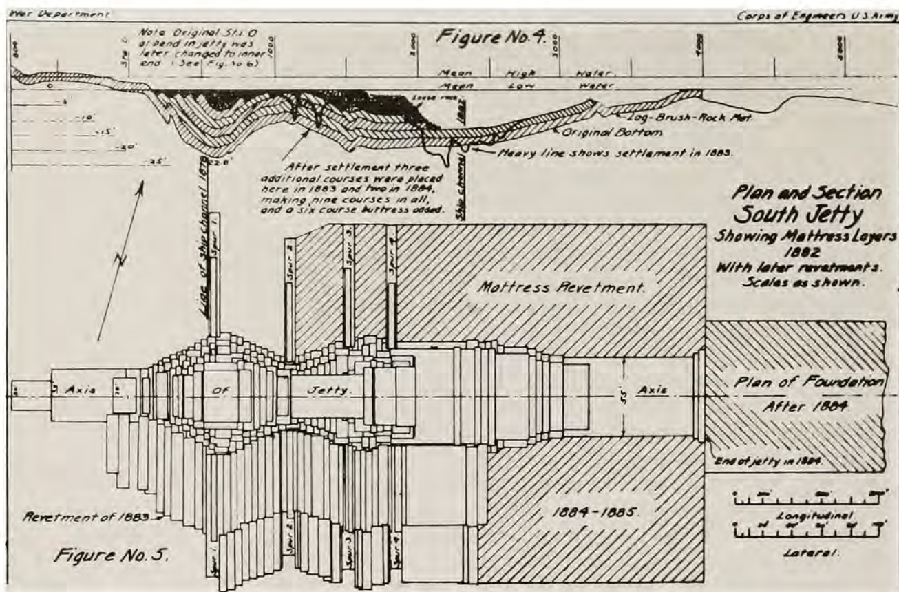
Plan of south jetty, 1882. Courtesy Corps of Engineers.
