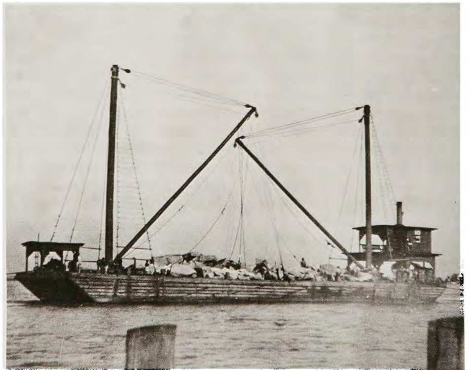
Workmen unload small pieces of stone onto jetty in 1900 (top). Another load of stone arrives for the jetties (bottom).
