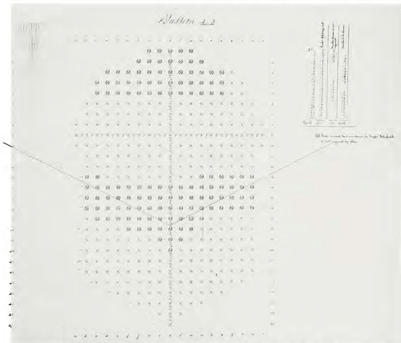
An 1848 status sheet from Major Sanders' log, showing the pile pattern for the bastion between fronts 2 and 3. The encircled piles were driven a decade previously by Major Delafield, according to the old plan. The new plan called for 387 piles, of which 256 remained to be driven.
