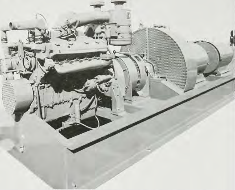
200 K. W. uninterrupted Power Generation set with control console. Eleven units were procured and installed at five Air Force Bases within the Continental U.S., as back-up equipment to provide uninterrupted power for the Air Warning System.
