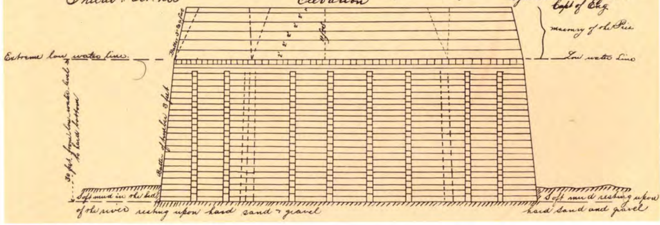
Plan, elevation and section of the piers designed as icebreakers for the harbor of New Castle, Delaware. Signed, Richard Delapfield, Captain of Engineers, Philadelphia, October 1835. —Historical Collection, Philadelphia District
