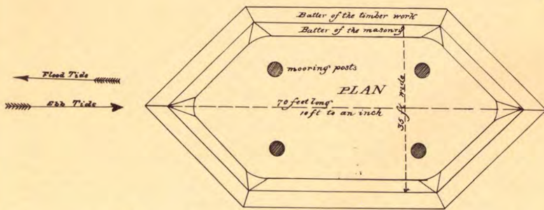
Plan, elevation and section of the Piers designed as Icebreakers for the Harbour of New Castle (Delaware) projected for the formation of said harbour according to the Act of the State of Delaware passing the harbour and others to the U.S and the Act of Congress accepting the cession Philad. Oct. 1835 Signed, Richard Delapfield Squad Road, Delapfield Capt of Eng.
