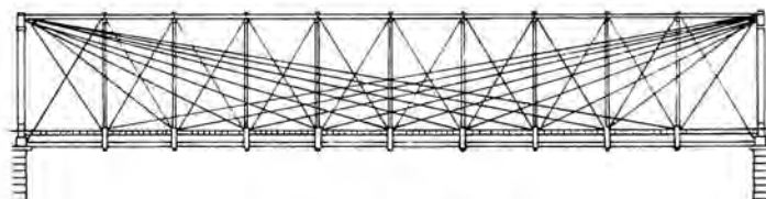
Bollman Truss
