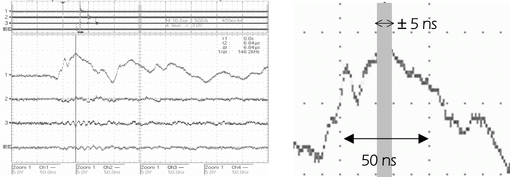
FIGURE 2: Screenshot of an X-ray pulse on an oscilloscope – close-up with accuracy range
