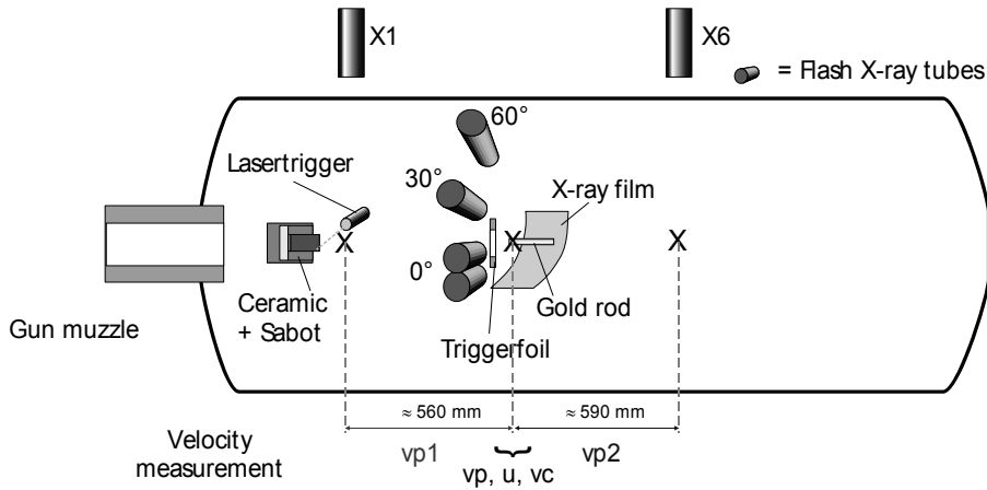
FIGURE 1: Test-set-up – reverse ballistic method
