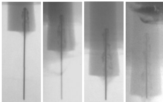
FIGURE 3: X-ray sequence for Exp. 2581 – Penetration and erosion data for several experiments
