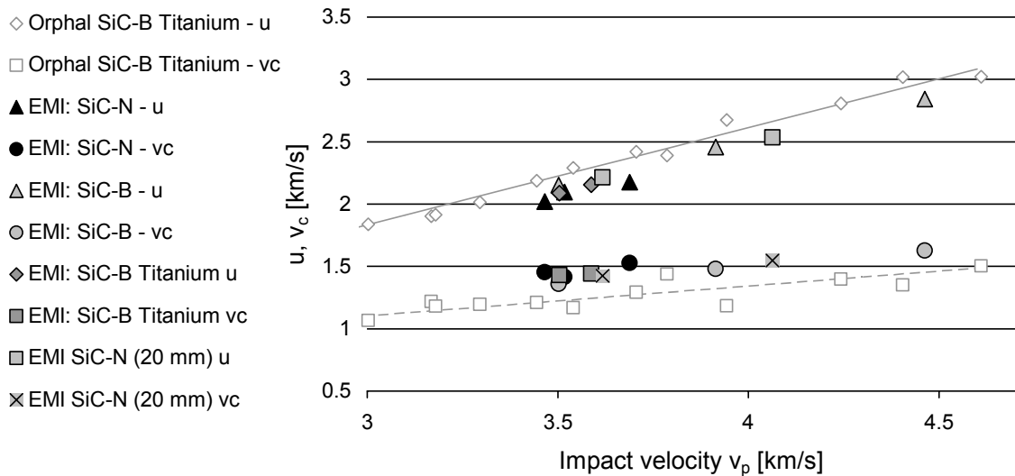
FIGURE 4: Penetration and consumption velocity as a function of impact velocity
