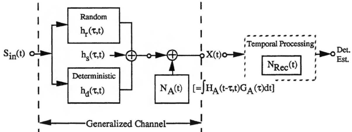
Figure 2.3 Purely temporal channel equivalent of the space-time generalized channel of Figures 2.1 and 2.2.
