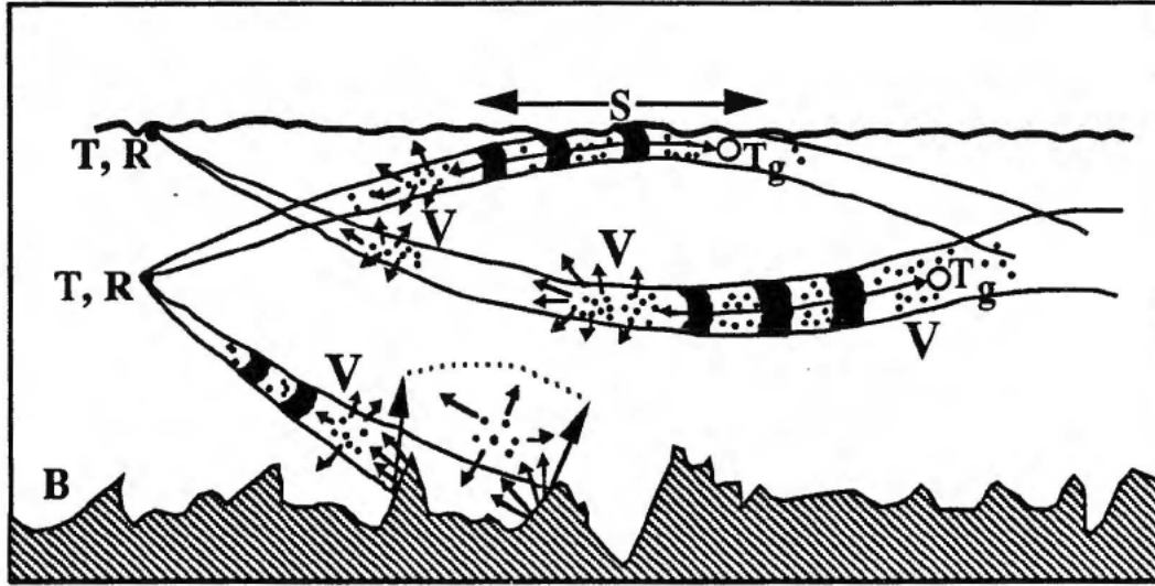
Figure 5.1 Sketch of some typical ("high-frequency" or n. b.) propagation of beamed signals, when \nabla c \neq 0 , showing potential mechanisms of reverberation: T, R = transmitter, receiver; T_g = target.
