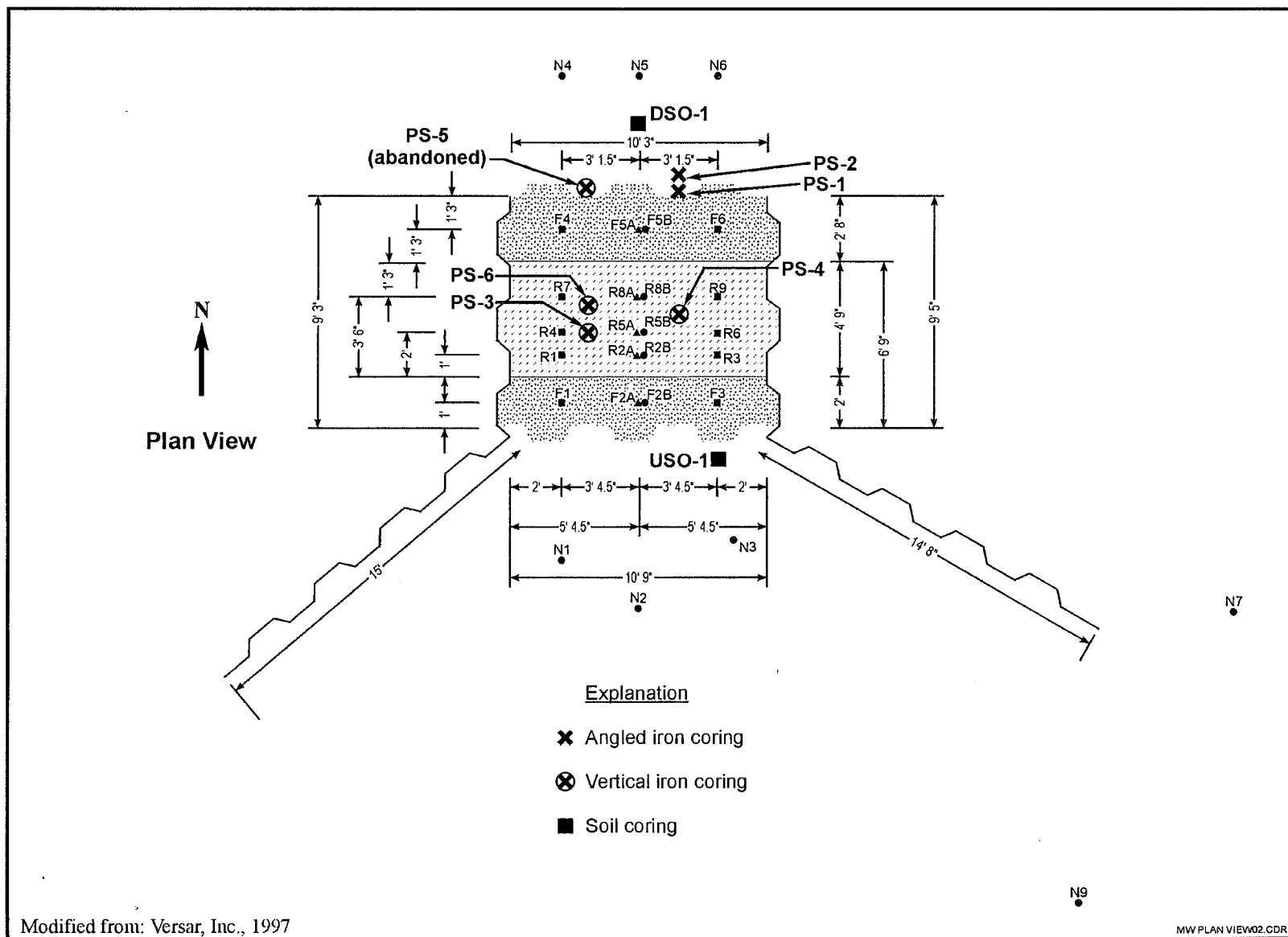
Figure 5-9. Sampling Well Locations in the PRB and Vicinity at Former Lowry AFB
