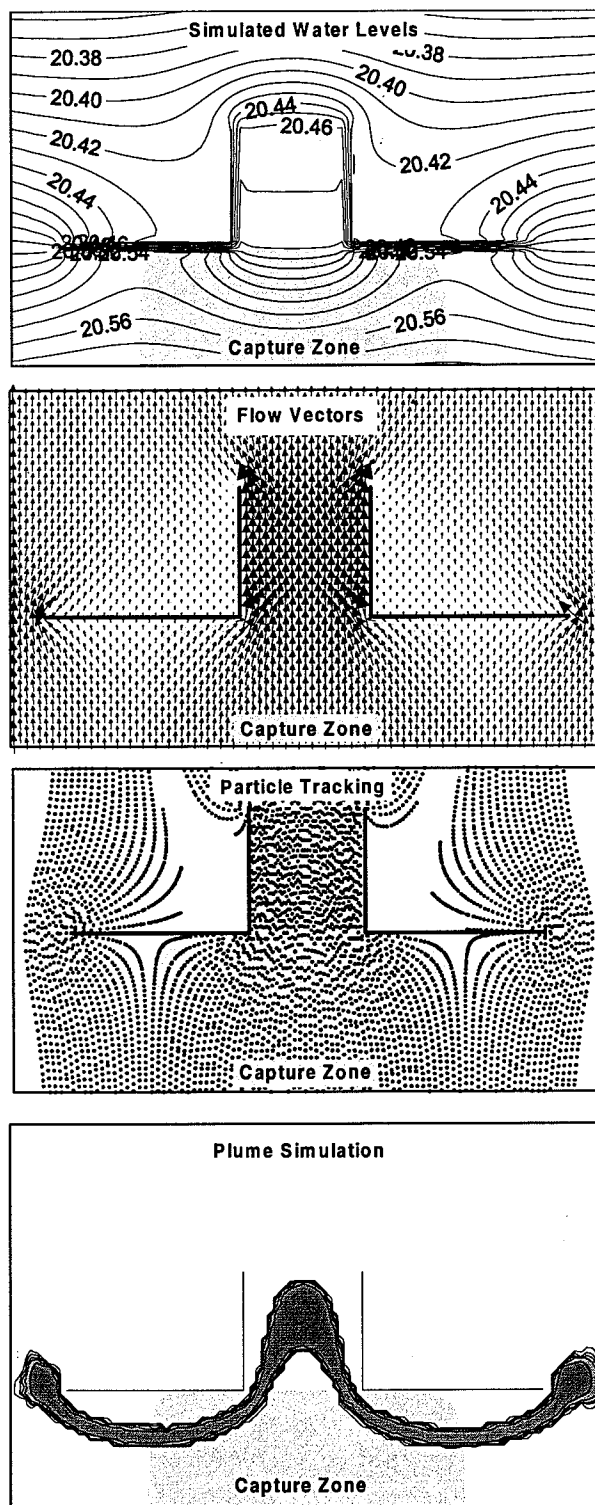
Figure 6-10. Modeling Methods Used to Illustrate Capture Zone of PRBs (Battelle, 2000c)
