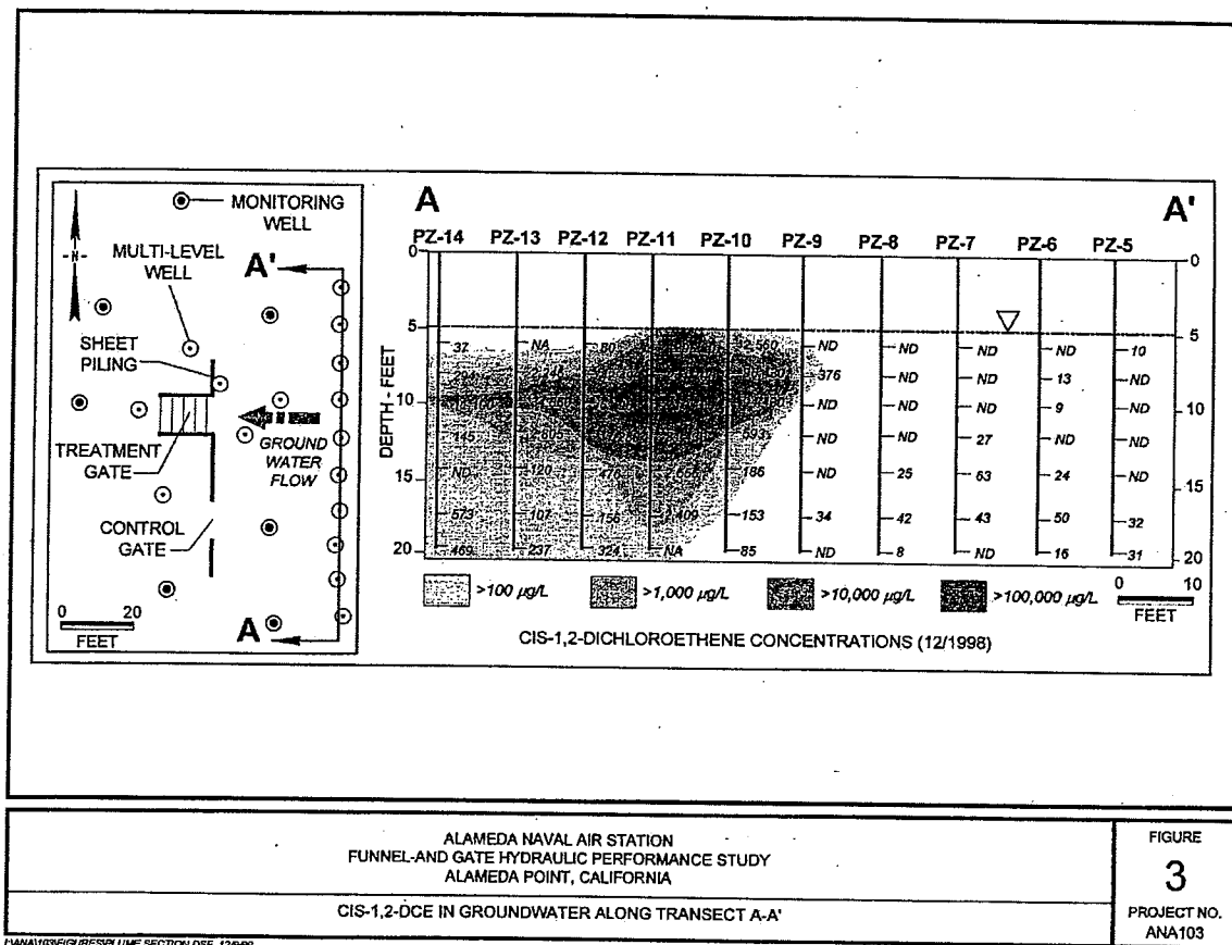
Figure 3-5. Schematic View of PRB and Upgradient Contamination Profile at Former NAS Alameda Site (Einarson et al., 2000)
