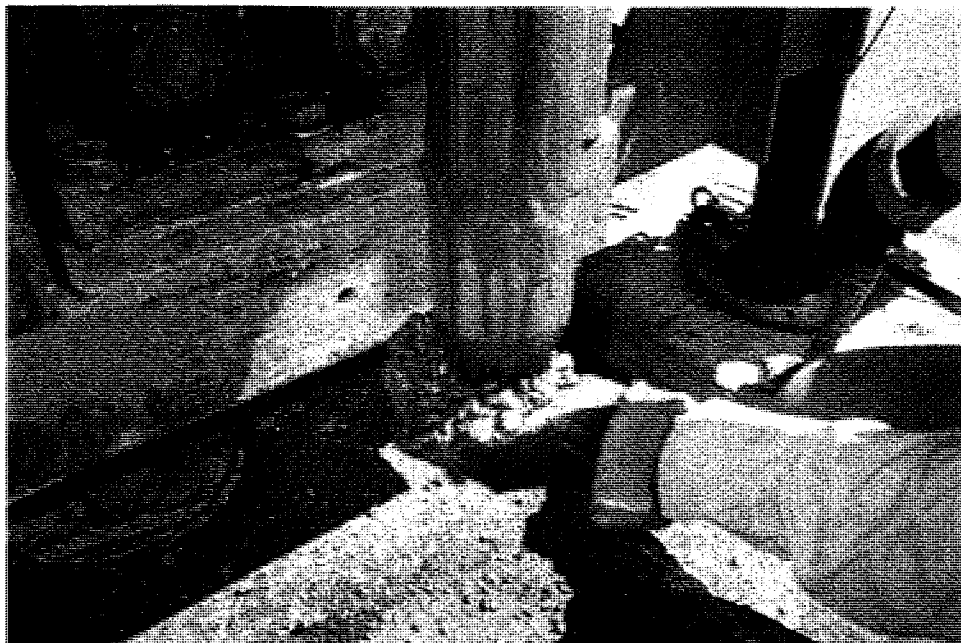
Figure 4-5. Pea Gravel Being Removed from Drive Casing
