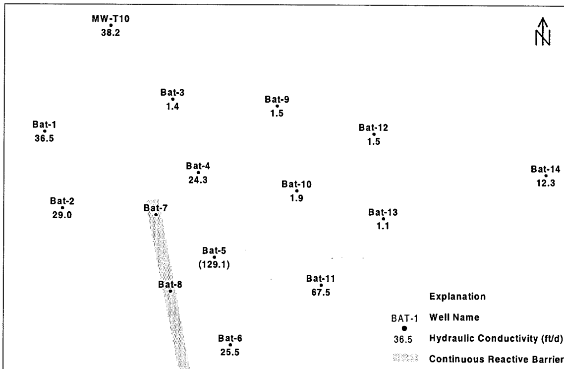
Figure 3-3. Hydraulic Conductivity Values (ft/d) from Slug Tests at the Seneca Army Depot CRB Showing Variations in Hydraulic Conductivity at the Site
