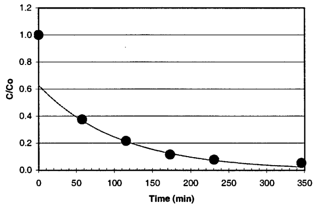
Moffett - TCE Profile 7 475 PVs
