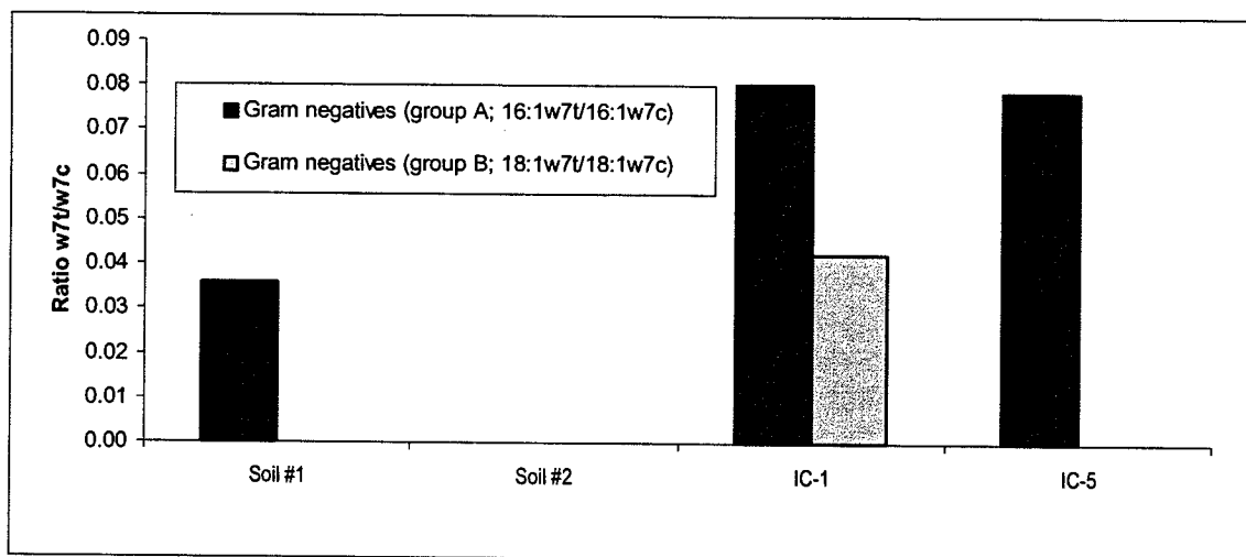
Figure4. Adaptation of the Gram-negative community to changes in the environment is determined by the ratio of \omega 7/\omega 7c fatty acids. Ratios (16:1 \omega 7/16:1\omega 7c and 18:1 \omega 7/18:1\omega 7c ) greater than 0.05 have been shown to indicate an adaptation to a toxic or stressful environment, resulting in decreased membrane permeability.
