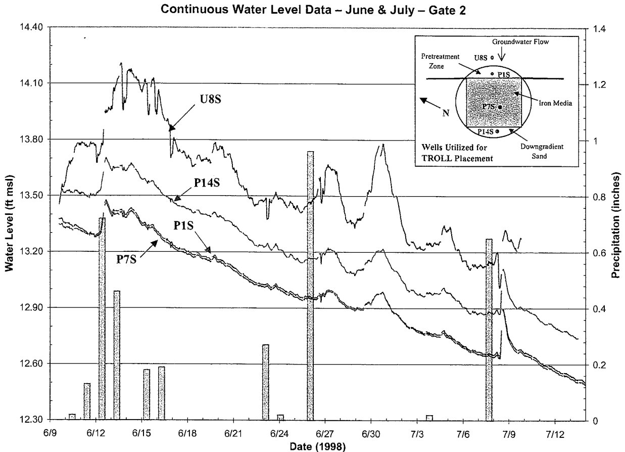
Figure 6-7. Example of Continuous Water Level Monitoring Data from Dover AFB PRB (Battelle 2000a)
