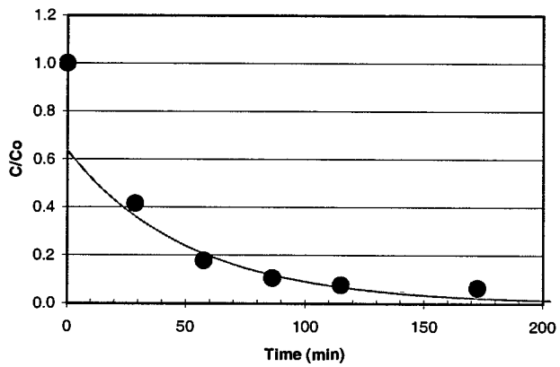
Moffett - TCE Profile 2 140 PVs
