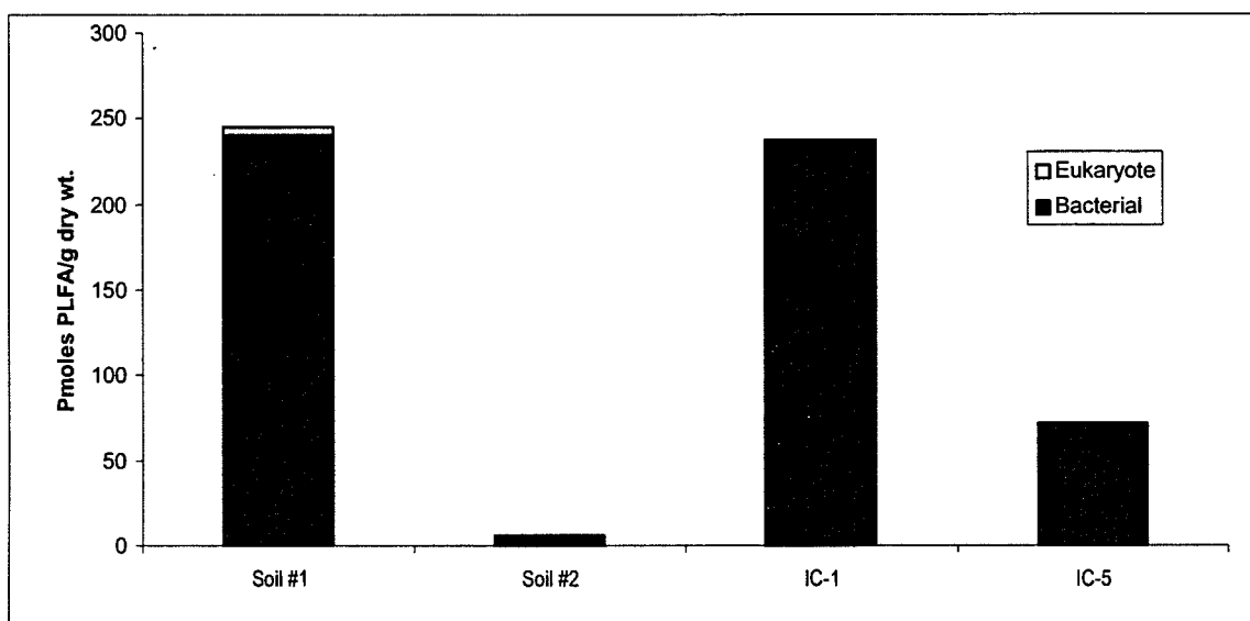
Figure1. Biomass content is presented as the total amount of phospholipid fatty acids (PLFA) present in a given sample. Bacterial biomass is calculated based upon PLFA attributed specifically to bacteria, whereas eukaryotic biomass is based on PLFA associated with higher organisms.
