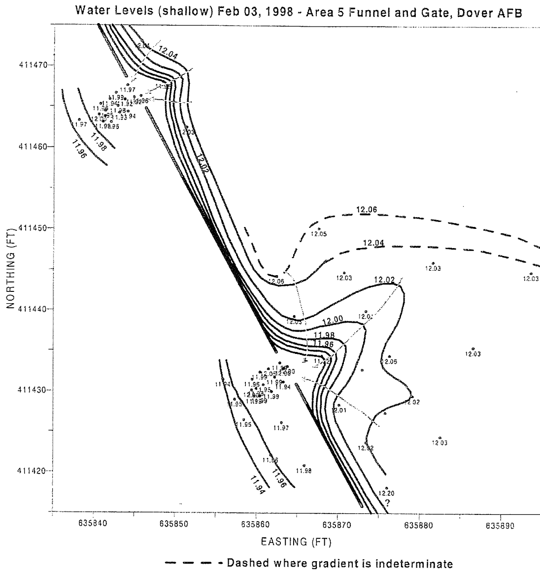
Figure 6-2. Water Levels and Flow Patterns at Dover AFB PRB Site for February 1998 (Battelle, 2000a)
