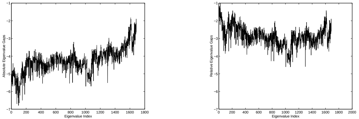
Figure 6.5: Absolute and Relative Eigenvalue Gaps for SiOSi 6
