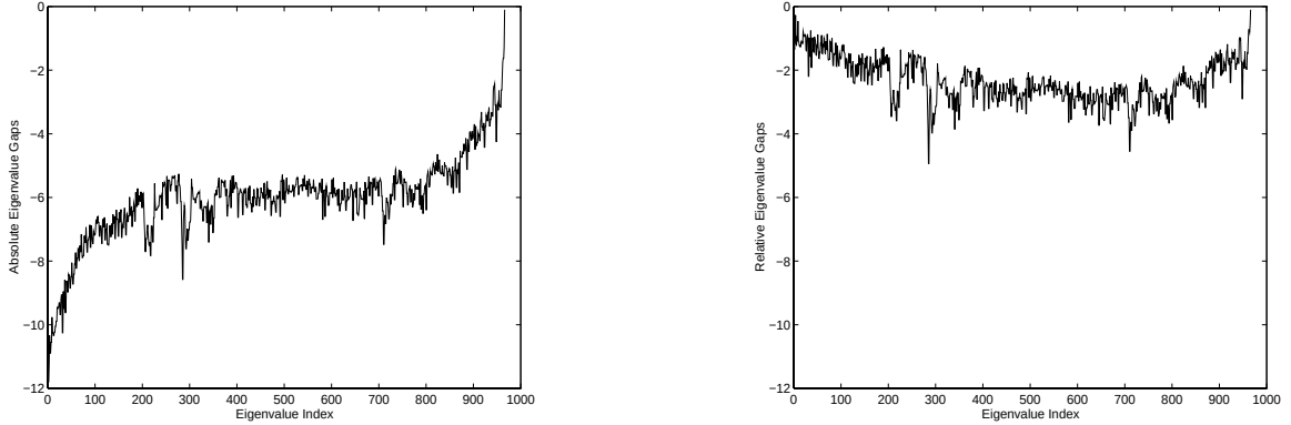
Figure 6.4: Absolute and Relative Eigenvalue Gaps for Biphenyl
