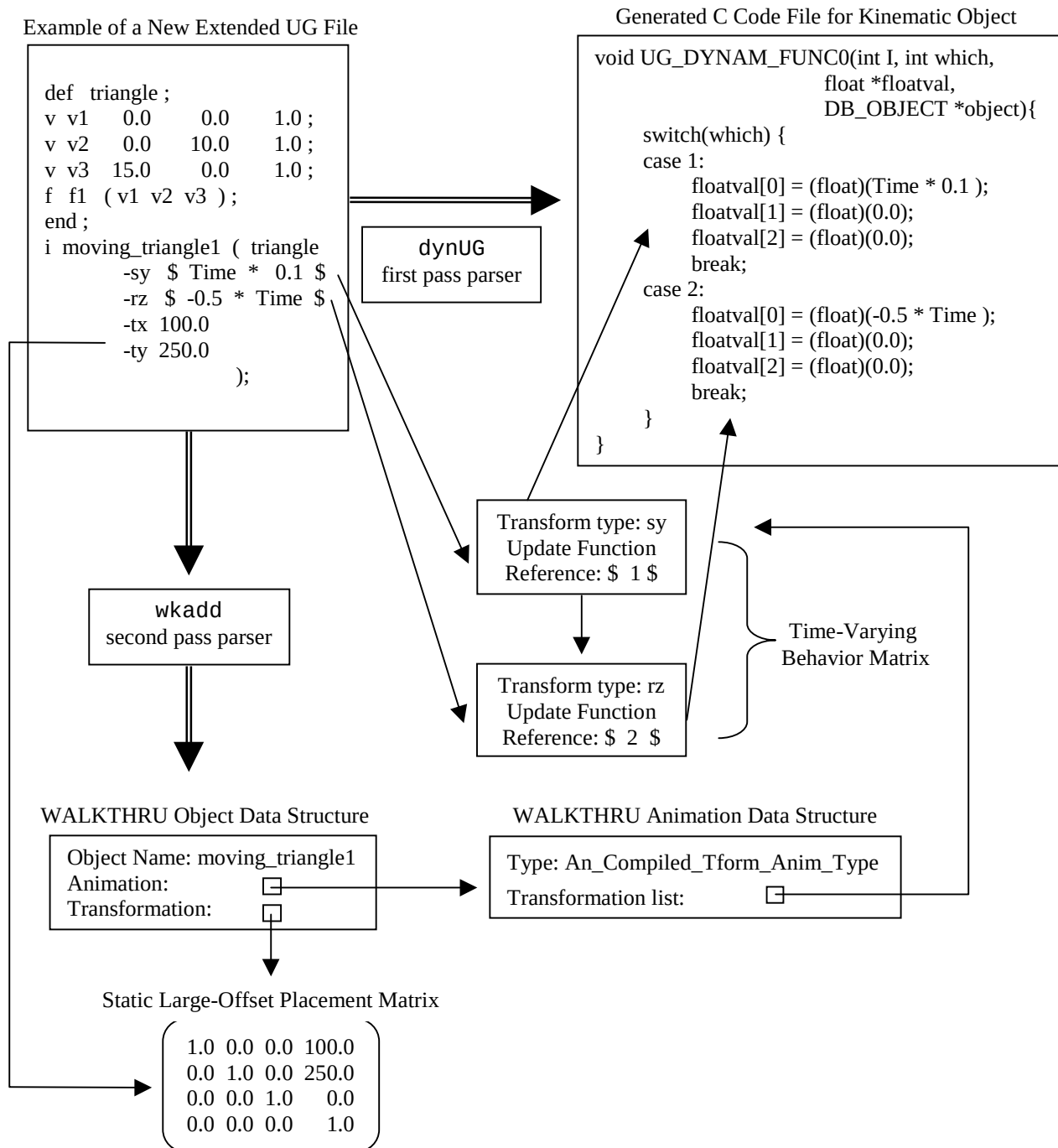
Figure 4.5: The process of creating a new compiled-code kinematic WALKTHRU object using the new wkadd and dynUG utilities
