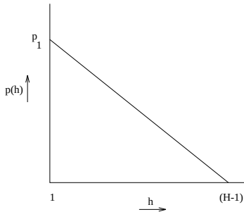
Figure 5: Probability distribution function p(h)
