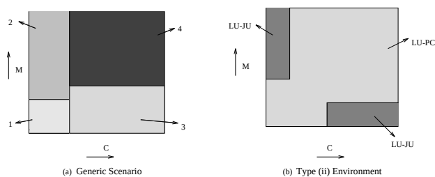
Figure 9: Partitioning of the M - C plane
