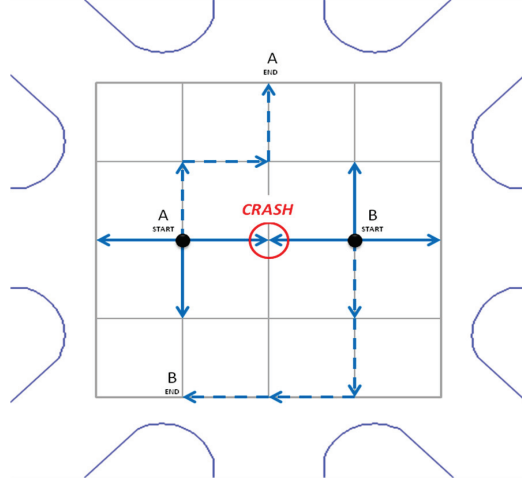
Figure 10: This figure represents the grid for multi-particle paths. Each particle is at one of the vertices of the grid and the motion of the particles is constrained along the grid. As an example the path of two particles is shown here. Collision of the two particles is restricted by not allowing them to share the same space at the same time.
