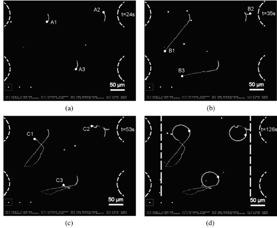
Figure 30: The control algorithm can correct for large errors in particle positions. This figure shows steering of three fluorescent beads (2.2 \mu\text{m} diameter, Duke Scientific) around three circles. At time t=24 s, corresponding to bead positions marked A1 , A2 , and A3 , the control was turned off for 11 s, allowing the particles to drift away (primarily due to the slow parasitic flow caused by surface tension forces at the reservoirs) by up to 150 \mu\text{m} . The control was then turned back on at t = 35 s (B1 , B2 , and B3 ), and the control algorithm steered the three original beads back to their desired positions (C1 , C2 , and C3 ). Four time instants are shown. (a) Right before control is turned off. (b) Right before control is turned back on (the three beads have drifted away a large distance). (c) At a time when the beads are back on track. (d) Final time when the beads have completed the remainder of their three circular paths (again to an accuracy of better than 1 \mu\text{m} ). The two straight lines in the last image illustrate the left and right boundaries of the control region. The control voltages scale with the size of the position errors. Position errors are very large and this would lead to very large control voltages. Therefore, the control scheme has been slightly modified: the control gain per particle is scaled in such a way that the voltage remains within the allowable [-10, +10] Volt range.
