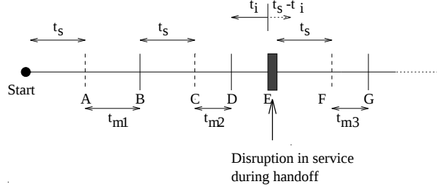
Figure 2: Probabilistic Guarantee
