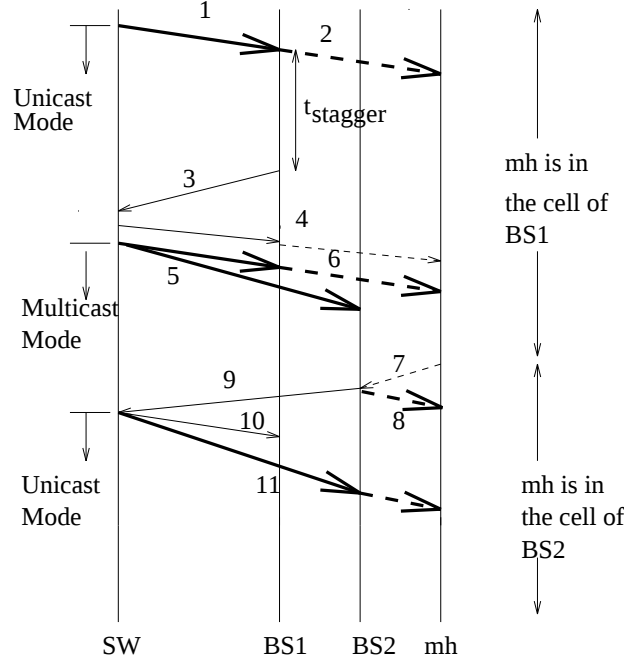
Figure 9: Connection Maintenance
