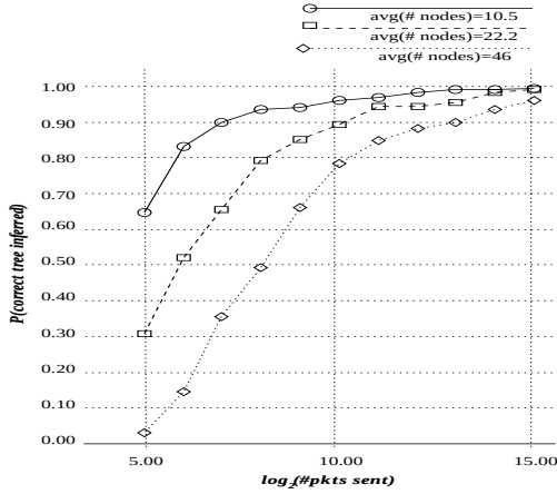
Figure 9: Binary trees: individual link loss rate is selected at random in the range [0%,10%]
