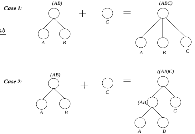
Figure 6: Possible relationships between a pair of nodes to be coalesced for arbitrary trees
