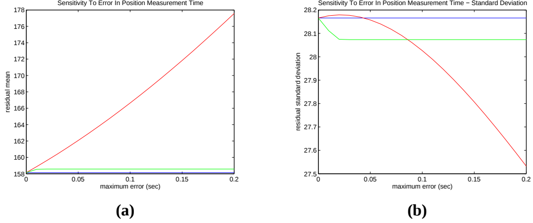
Figure 5.1: Mean (a) and standard deviation (b) of \min_x \|\bar{A}x - b\|_2 (blue), \max_{A \in A_\rho} \|Ax^{LS} - b\|_2 (red), and \min_x \max_{A \in A_\rho} \|Ax - b\|_2 (green) for different magnitudes of error in the times of the GPS/INS position measurements. Note that \min_x \|\bar{A}x - b\|_2 is independent of the maximum error \rho ; it is included for comparison.
