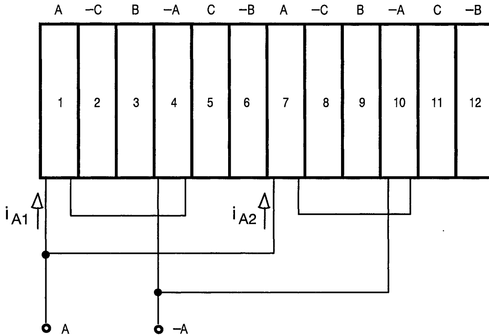
Fig. 4: Terminal connection of one phase of the LIL section
