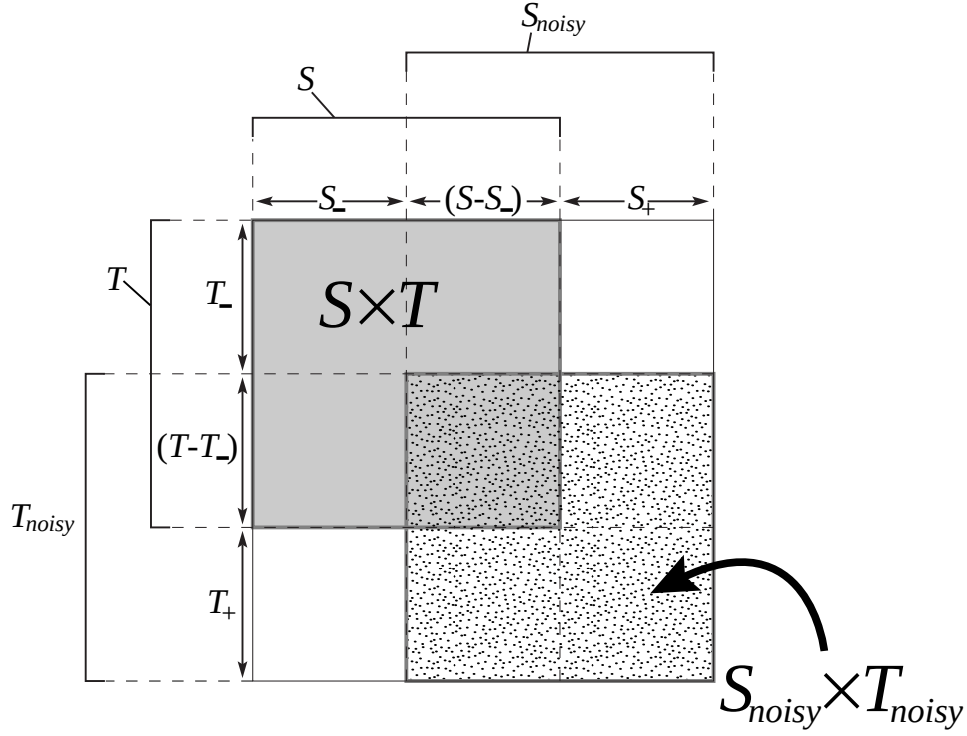
Figure A.1: Intuitive version of the differential cross product definition. The large square represents the tuples in the cross-product of (S + S_+) with (T + T_+) , borrowing a visual metaphor from Ripple Join [46]. The smaller shaded square inside the large square represents the cross product of the original relations S and T . The speckled square represents the cross product of these two relations after the tuples in S_- and T_- are removed and the tuples in S_+ and T_+ are added to S and T , respectively. The differential cross product computes the difference between these two cross products. Note that S_{noisy} - S_+ = S - S_- .
