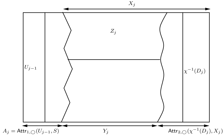
Figure 1: The sets of the construction.
