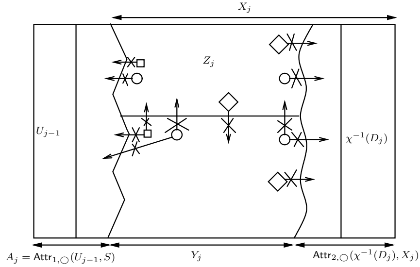
Figure 2: The sets of the construction with forbidden edges.
