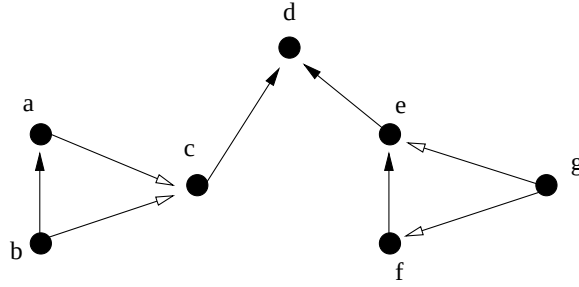
Figure 2.8. An Example Diposet
