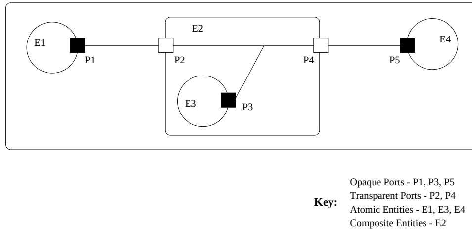
Figure 4.2. A Sample Ptolemy II Graph
