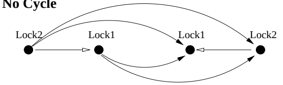
Figure 2.15. Order/Containment Constraints That Do Not Lead To Deadlock
