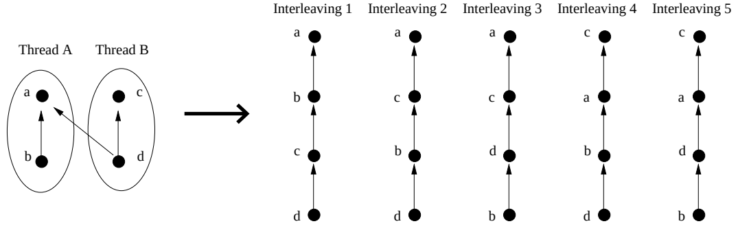
Figure 2.2. Sequential Interleavings
