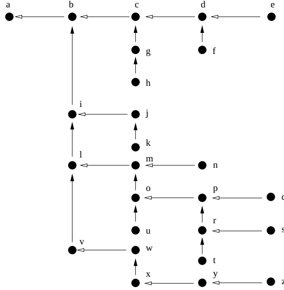
Figure 1.1. A Sequential Nested Diposet
