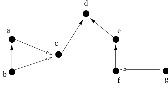
Figure 2.9. An Example Nested Diposet
