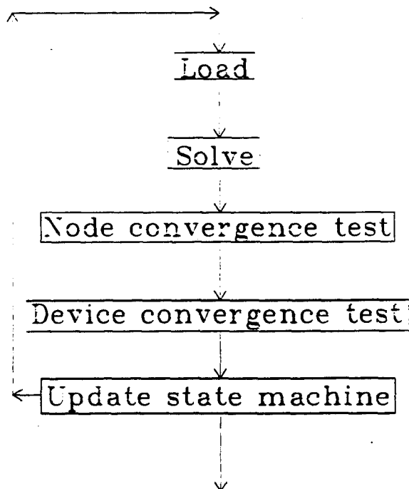
Figure 2.16 SPICE3 Newton-Raphson loop
