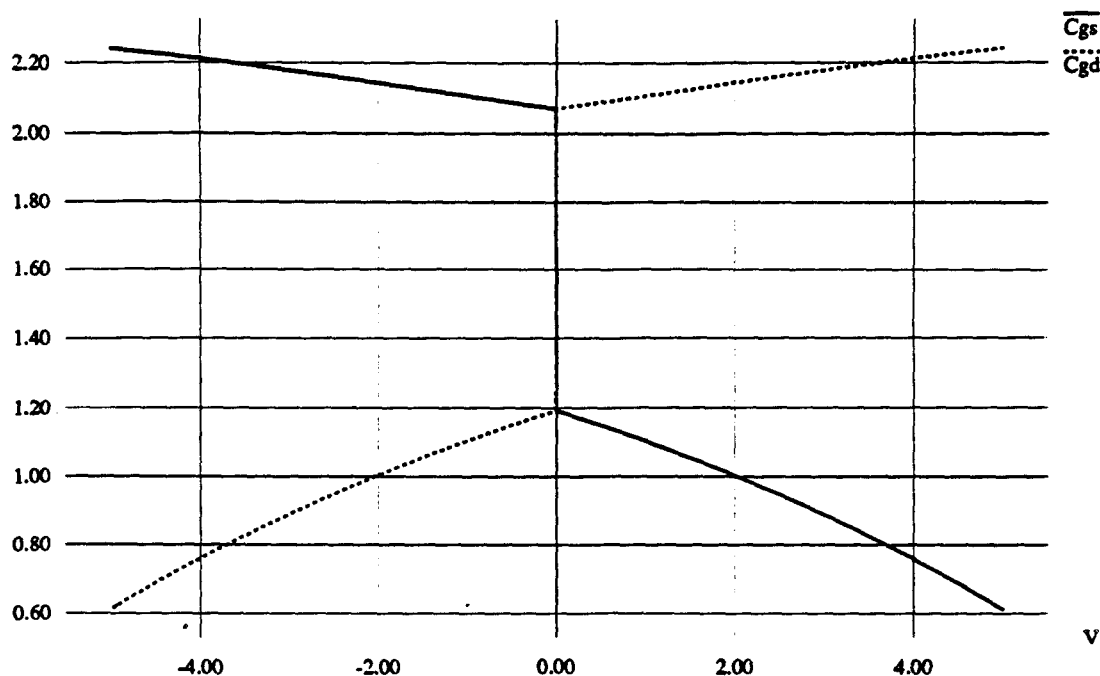
Figure 3.4 Gate-Source and Gate-Drain capacitance vs V ds before correction
