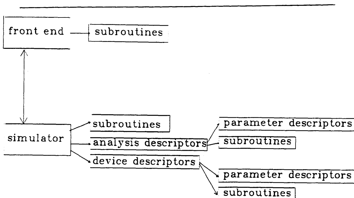
Figure 4.2 Descriptive data structure design
