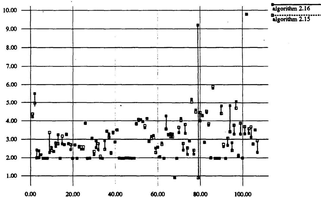
Figure 2.17 Comparison of iterations/timepoint for algorithms of Figures 2.15 and 2.16
