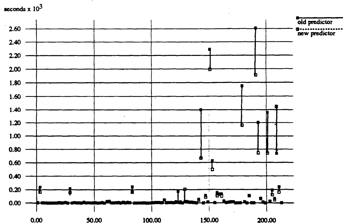
Figure 2.9 Performance gain from the use of a better predictor
