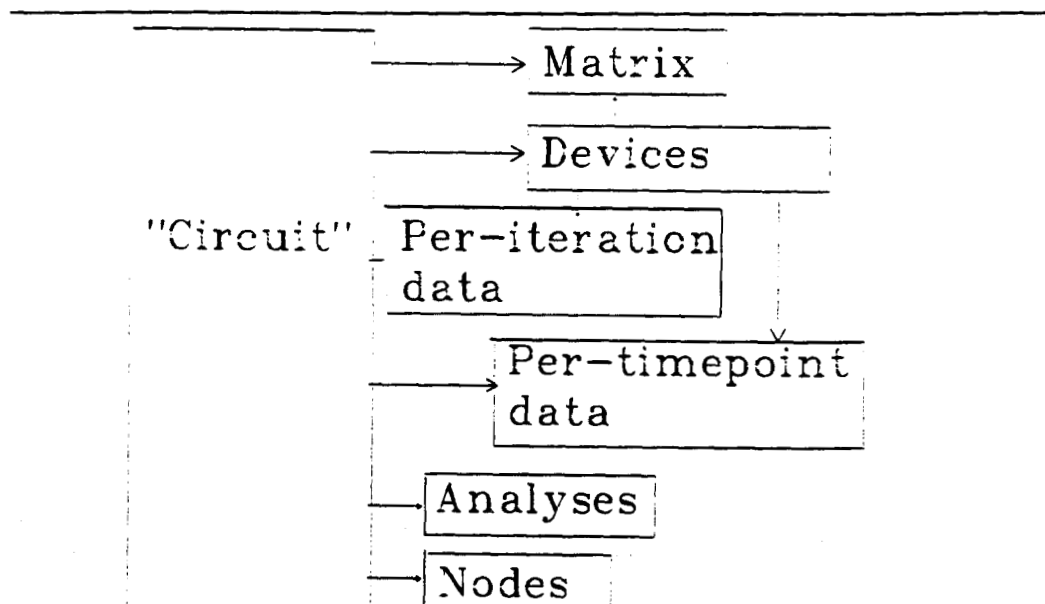
Figure 4.3 Local data hiding structure
