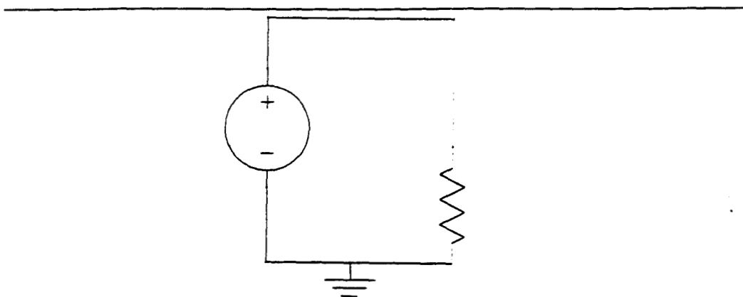
Figure 3.6 Voltage source causing MNA problems
