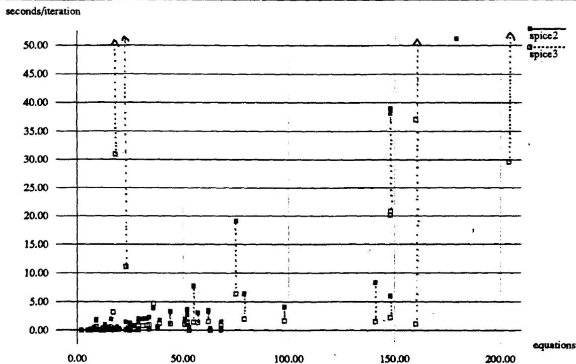
Figure 2.5 Matrix solve time versus number of equations for SPICE2 and SPICE3.
