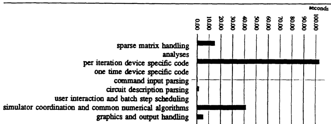
Figure 2.1 CPU time distribution for circuit N116DT
