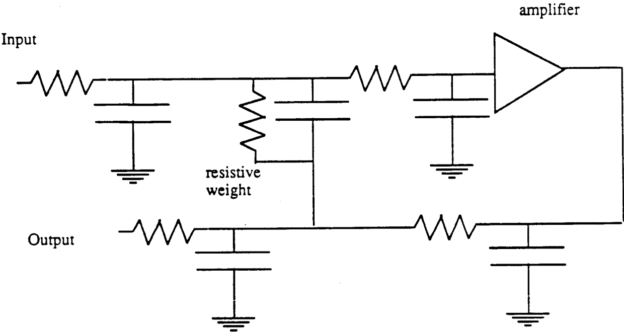
Schematic of one neuron:
