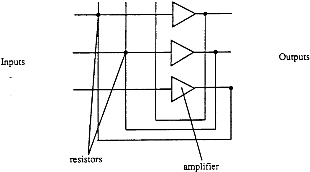
Basic schematic of Hopfield neural network:
