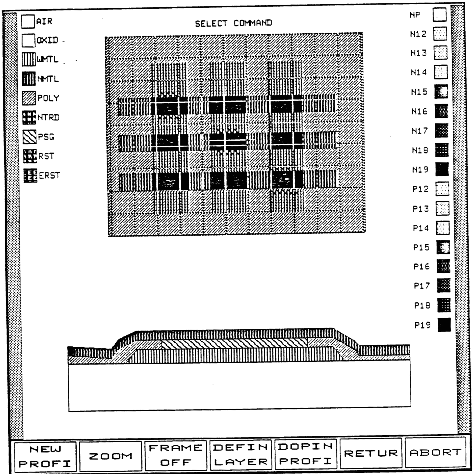
Figure 5.2. One interconnect element of a VLSI Hopfield Neural network.
