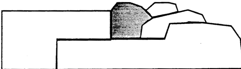
Case 3. Multiple polygons with vertexes equal to highest point in surface.
