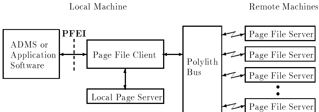
Figure 1: Overview of the components of the Page File data type.
