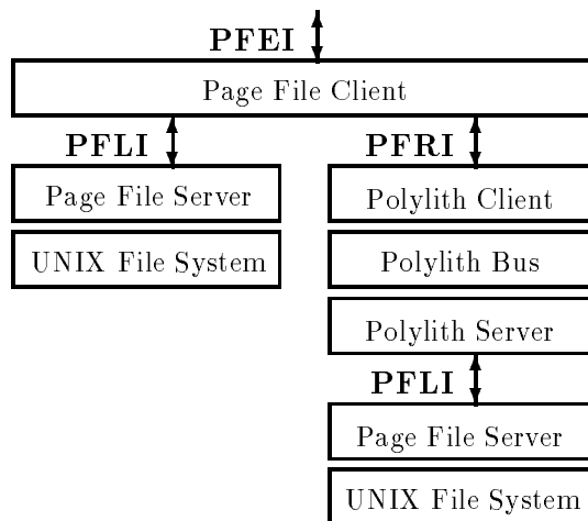
Figure 3: Software modules and interfaces.
