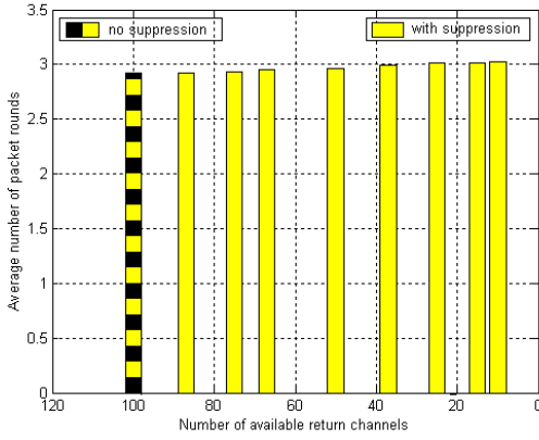
Fig. 2. Number of packet rounds versus number of available return channels for a set of R = 100 receivers.
