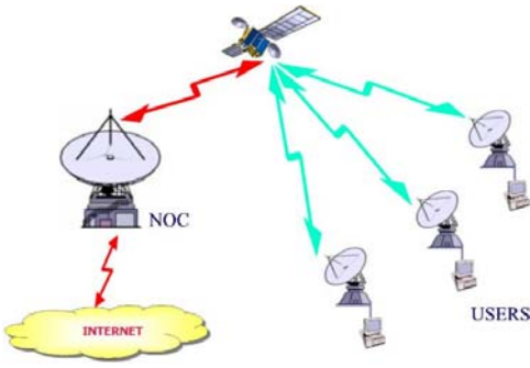
Fig. 1. Network Architecture
