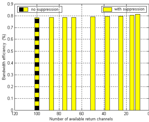
Fig. 3. Bandwidth efficiency as a function of number of available return channels for a set of R = 100 receivers.
