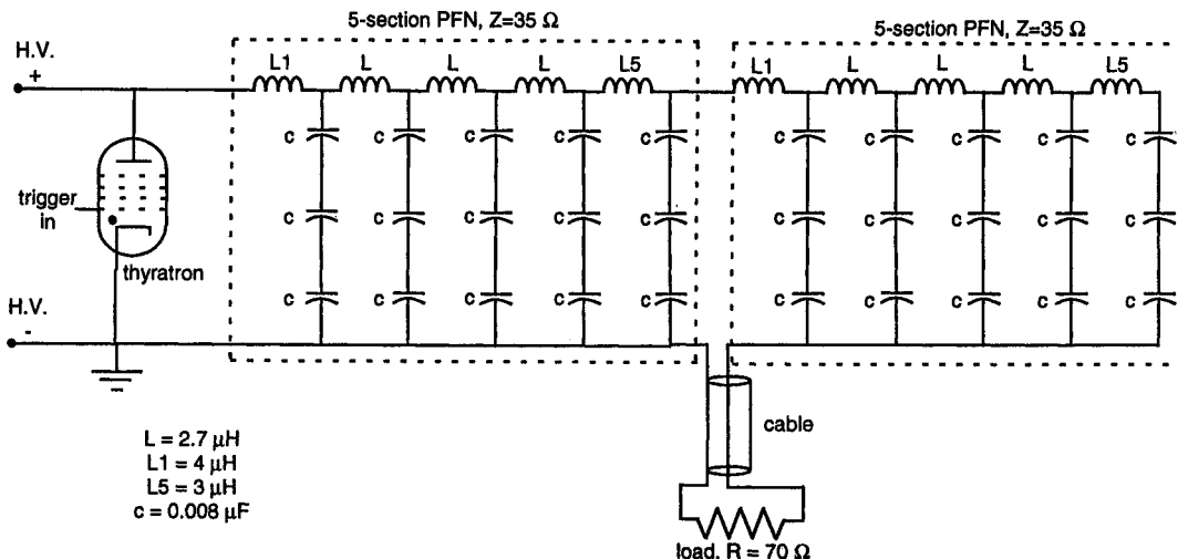
Figure 1. Circuit schematic for Blumlein pulser consisting of two 35-Ω PFL's.
