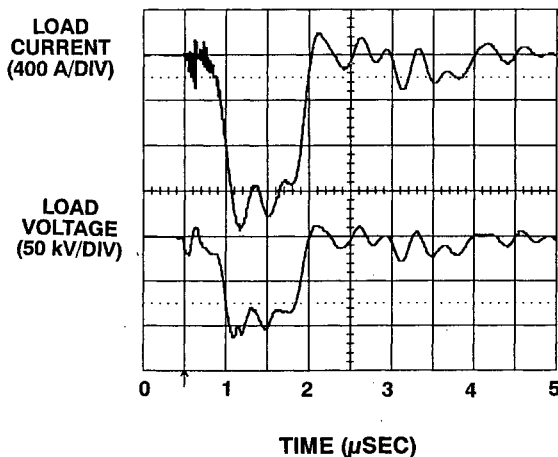
Figure 4. Voltage and current delivered to 70-Ω resistive load for a network bias of 100-kV. PFL inductor taps not optimized for flattest pulse. Arrow on time axis indicates firing of thyatron.
