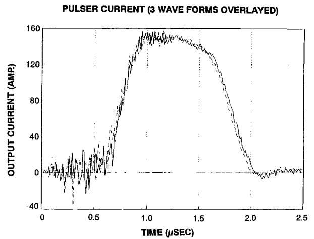
Figure 6. Three current pulses at 70-Ω resistive load overlaid. Note pulse reproducibility.
