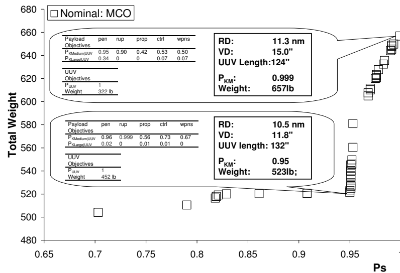
Figure 4.7 UUV-Payload nominal optimal designs in deterministic case
