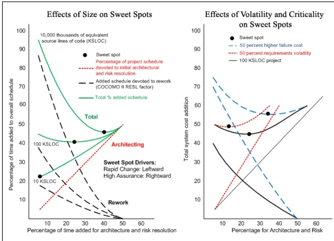
Figure 2. Architecture Evidence Shortfall Penalties and Resulting Architecting Investment Sweet Spots
