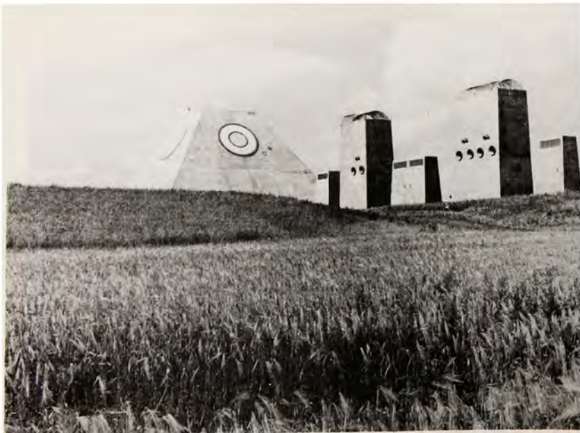
THE TURRET OF THE MSCB and the intake and exhaust stacks of the underground power plant.
