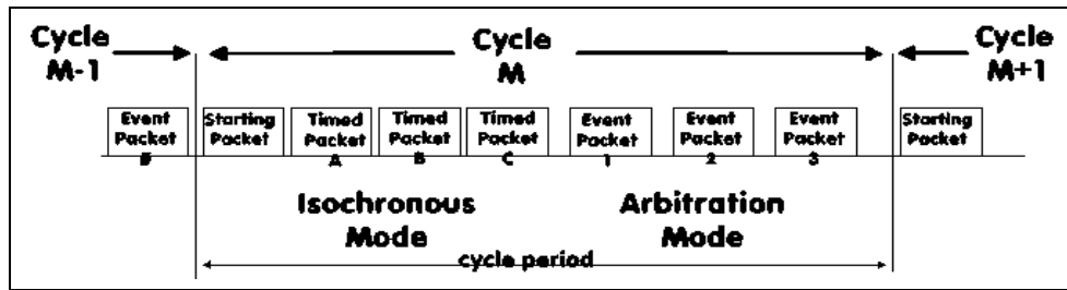
Figure 6 - Isochronous Mode
