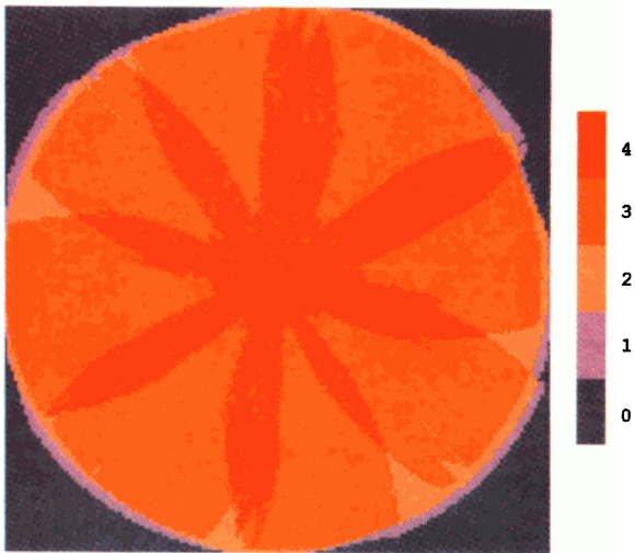
FIG. 5. The number of reverberation maps available per grid point, \Omega .
