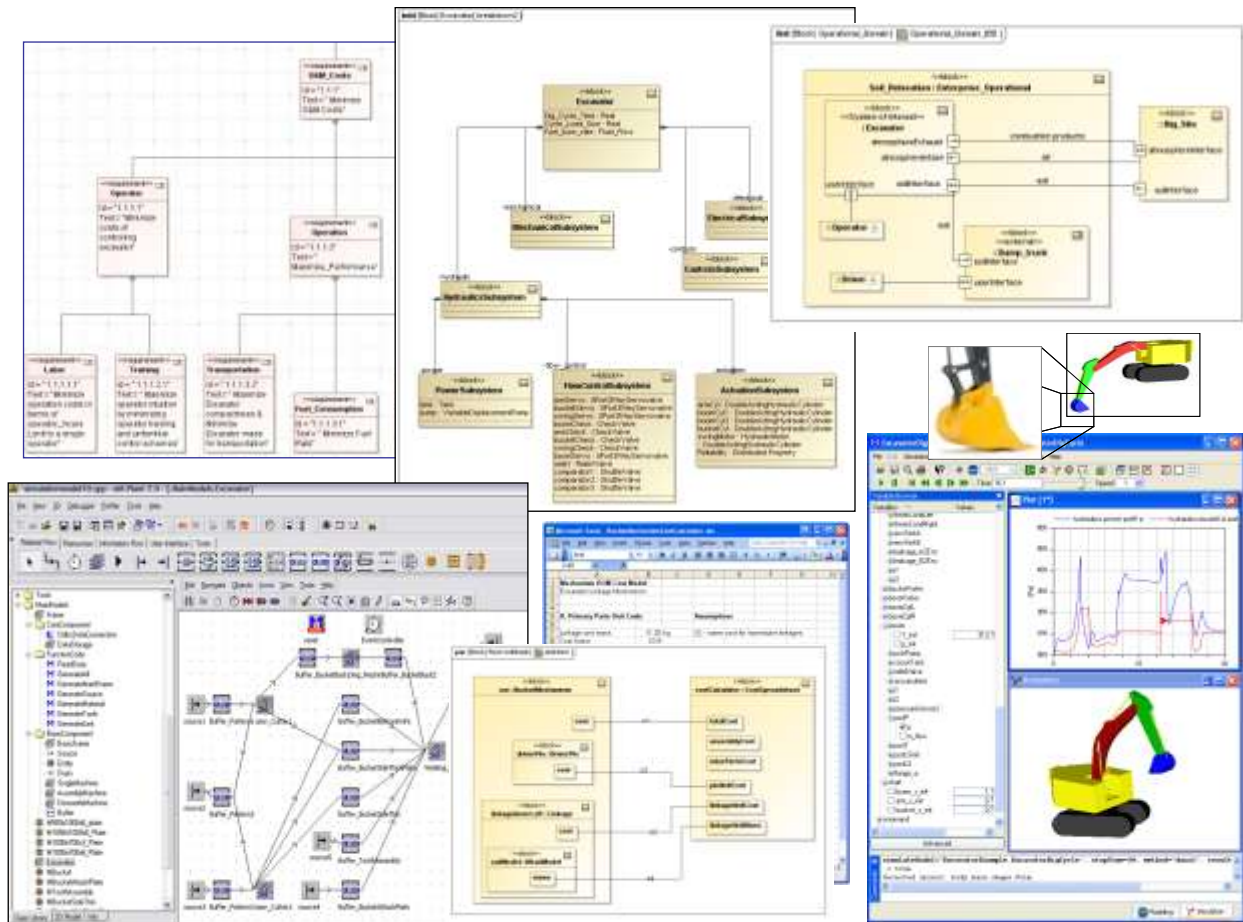
Figure 2 – Excavator testbed: sample SysML diagrams and native solver models.
