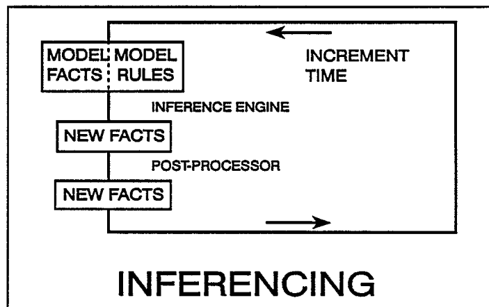
Figure 2 - Inferencing Model
