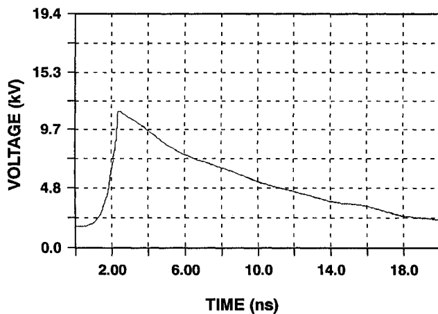
Figure 3 Output pulse width no interruption.
