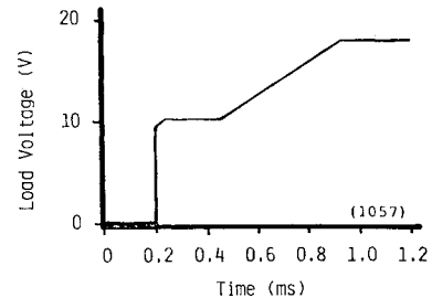
Fig 6. Detail of Commutation Voltage
