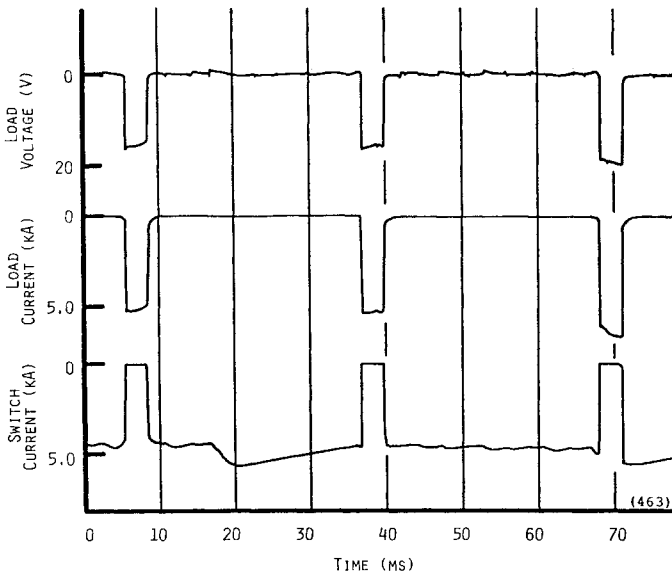
Fig 5. Typical Commutation Events
