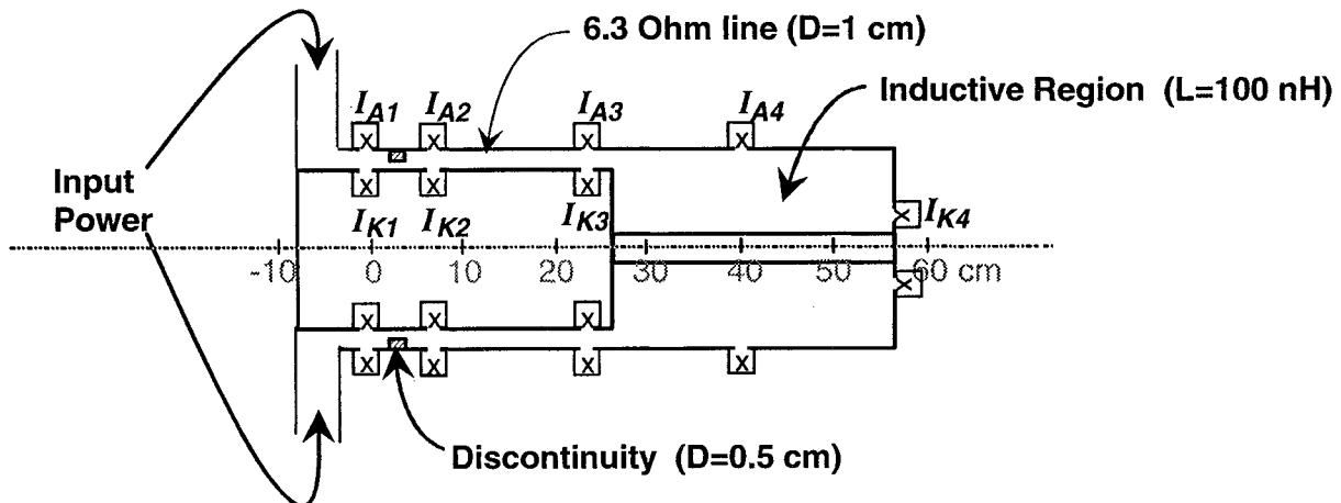
Figure 1. Schematic of the Gamble II power-flow hardware.
