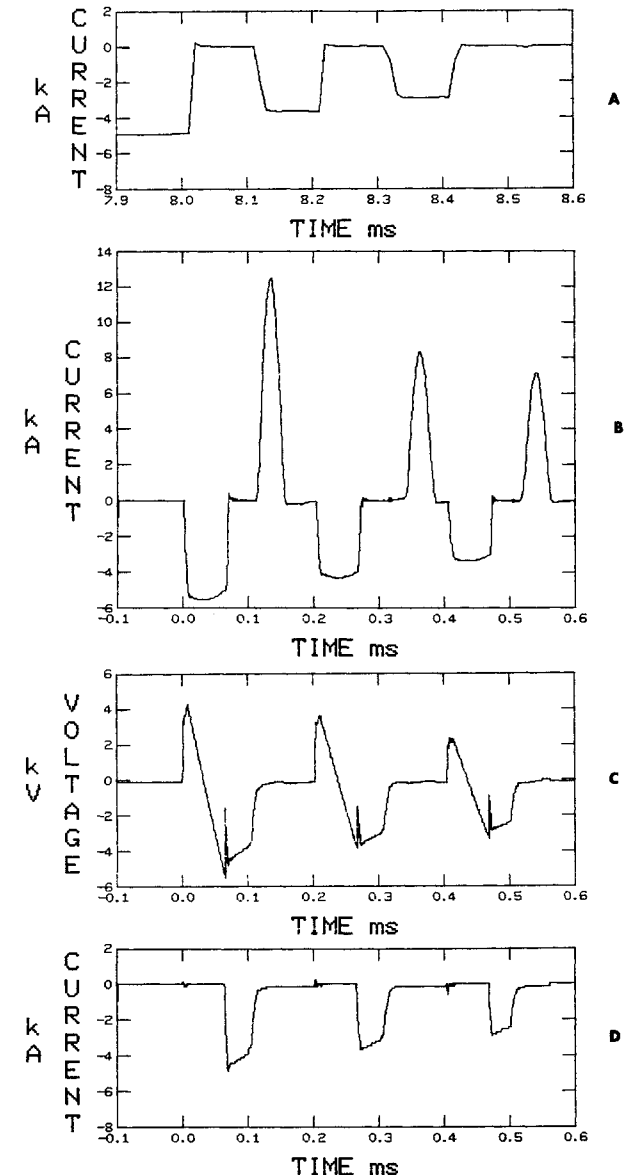
Fig. 5. Voltage and current waveforms showing 23-MW, 5-kHz operation of repetitive pulse circuit.
