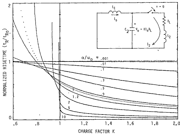
Fig. 9. Normalized risetime plot vs. voltage factor.
