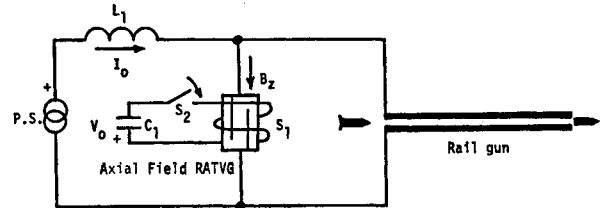
Fig. 10. Repetitive railgun using axial field RATVG.
