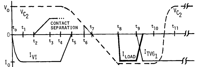
Fig. 4. Simplified waveform representations of repetitive transfer circuit operation.
