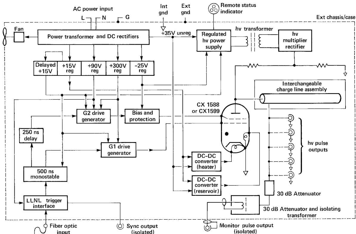
UNIT BLOCK DIAGRAM
