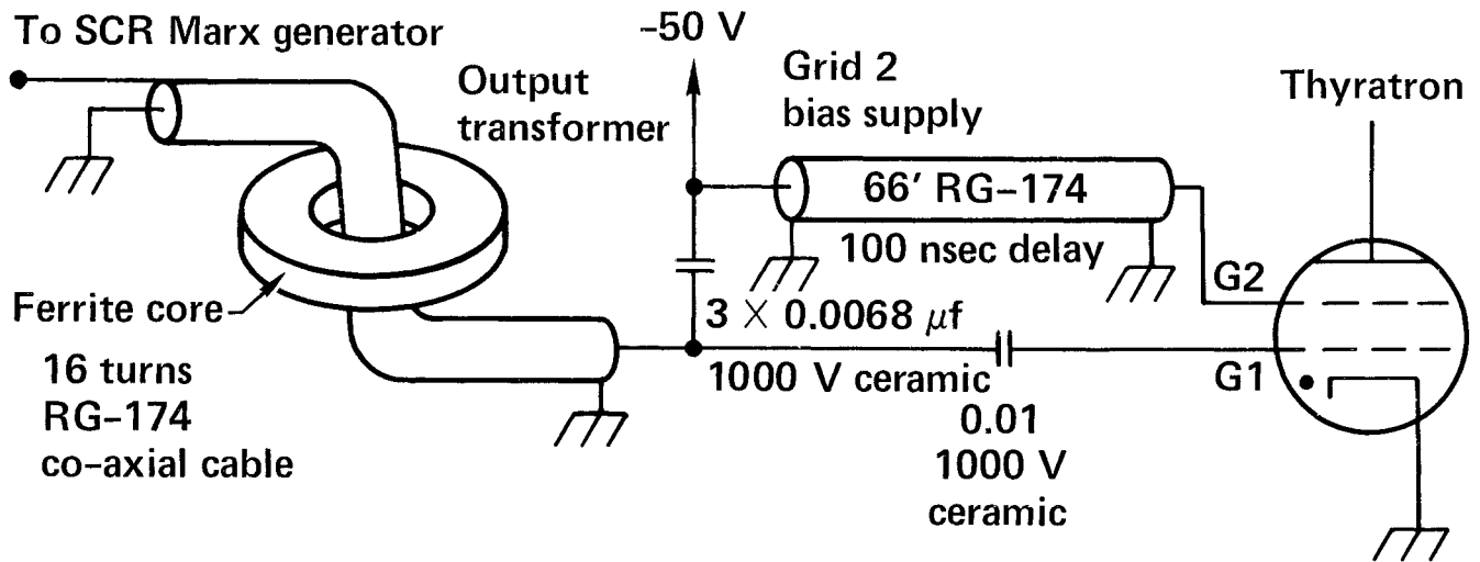
FIGURE 4 DRIVING TETRODE THYRATRONS
