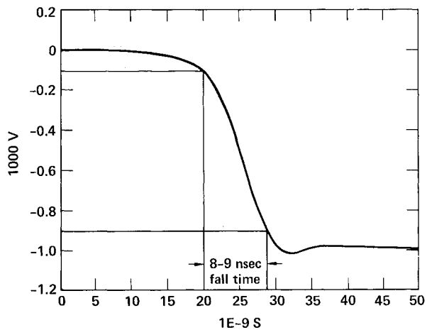
FIGURE 2A OUTPUT WAVEFORM
