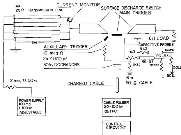
Fig. 2. Experimental Setup
