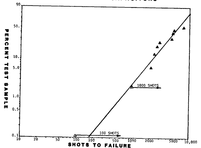
Figure 3. Lifetime data for SHIVA STAR capacitors.
