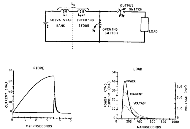
Figure 6. Inductive pulse compression circuit and circuit performance.
