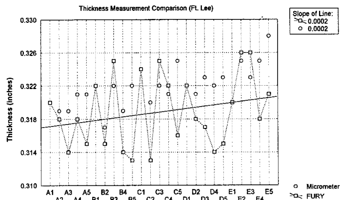
Figure 5. End Cap Mechanical vs. Fury Thickness Measurement
