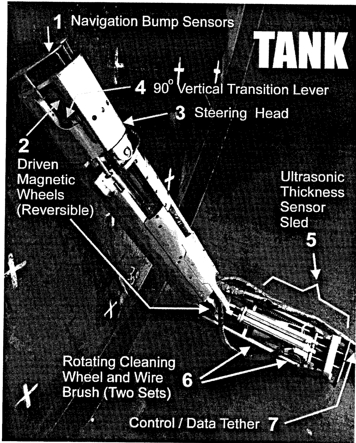
Figure 1: Photograph of Fury Robot
