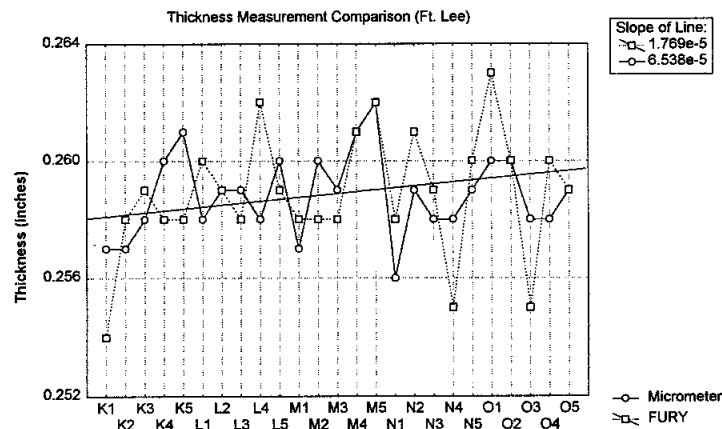
Figure 4. Bottom, Quarter Mechanical vs. Fury Thickness Measurement
