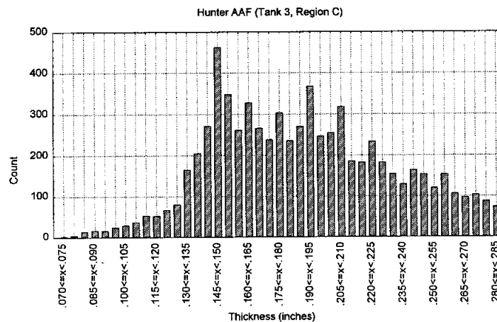
Figure 8. Thickness Distribution Region C in Tank 3 (Figure 5)
