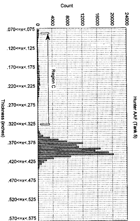
Figure 11. Tank 5 Thickness Distribution
