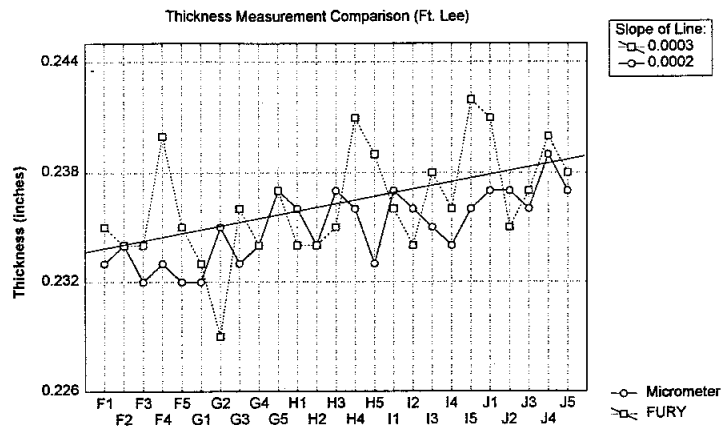
Figure 3. Bottom, Middle Mechanical vs. Fury Thickness Measurement
