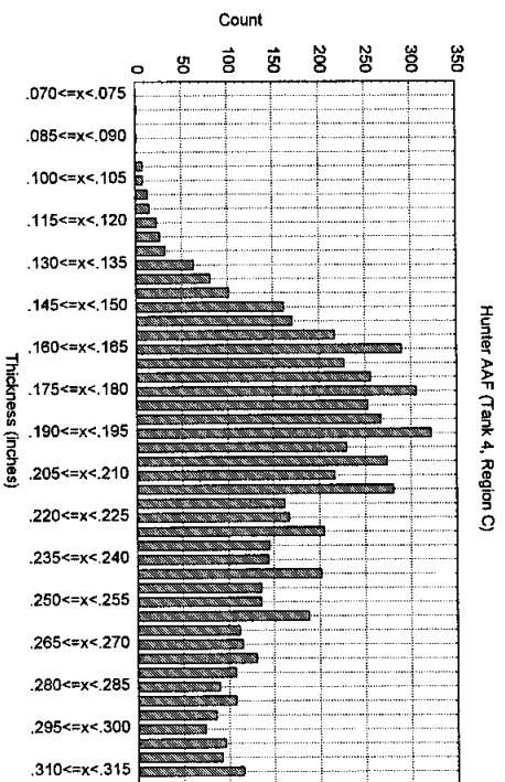
Figure 10. Region C Thickness Distribution in Tank 4 (Figure 7)
