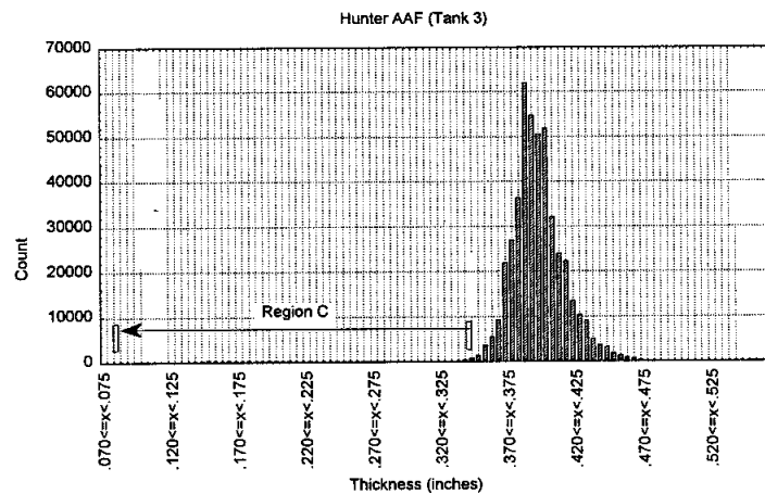
Figure 7. Thickness Distribution in Tank 3
