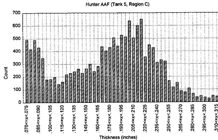
Figure 12. Region C Thickness Distribution Tank 5, (Figure 9)
