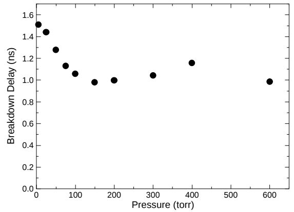
Figure 6. Breakdown delay with pos. needle, radial geometry, at 14 kV in argon as function of pressure
