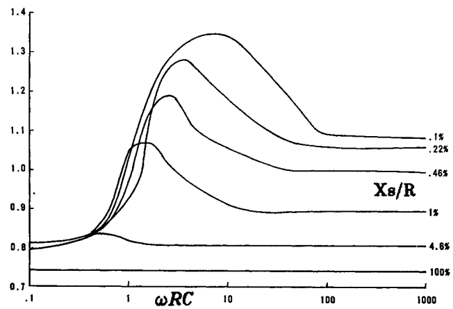
Figure 5 Normalized RMS Line Current vs \omega RC
