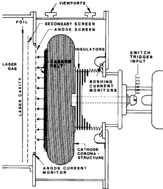
Fig. 2. Representative electron gun cross section for the Aurora e-guns. The LAM employs two PFLs for each of its e-guns in a double-sided excitation arrangement to achieve uniform pumping across its large laser aperture.
