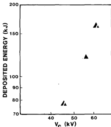
Fig. 5. Measured e-beam energy deposition into the LAM laser gas as a function of Marx charge voltage.
