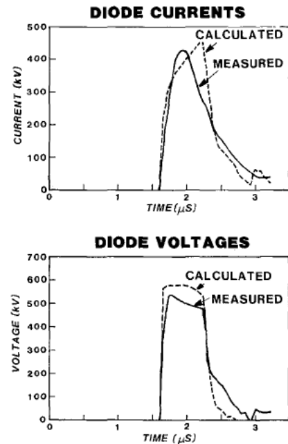
Fig. 3. Comparison of calculated (NET-2) and measured waveforms for the LAM cathode voltage and current. The PFL charge voltage was 1.16 MV at a switchout time of 1.8 \mu s. This switchout time is approximately 2 PFL transit times before the peak PFL ringup voltage.
