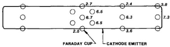
Fig. 4. Preliminary measurements of the spatial distribution of the preamplifier cathode current density. Operation at higher voltages and B fields is expected to produce a more uniform distribution.
