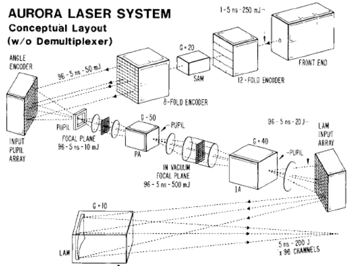
Fig. 1. Conceptual block diagram of the Aurora laser system not including the target details.
