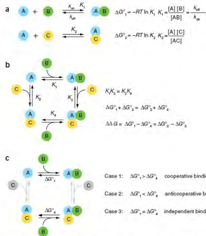
Figure 1 Thermodynamic cycles and cooperativity. (a) Hypothetical set of bimolecular complexes between component A and two other components (B and C), with the rate constants, equilibrium constants and free energies for complex formation. (b) A thermodynamic cycle for formation of the ternary complex ABC by two different possible routes: either B binds first, or C binds first. There are four equilibrium constants that describe the formation of the various complexes. Because they converge on the common product ABC, the thermodynamics must be independent of the pathway chosen around the cycle, and constraints are placed on the relative values of the equilibrium constants and hence the free energies. The thermodynamic coupling free energy ( \Delta \Delta G ) gives the difference between binding of one component in the presence of the other. (c) Definition of cooperativity in terms of binding of B in the presence or absence of C. The two vertical binding reactions are gray to emphasize the comparison of \Delta G^{\circ}_1 and \Delta G^{\circ}_4 . If B binds better in the presence of C, the binding is cooperative. If B binds worse in the presence of C, the binding is anticooperative. In the third case, binding of B is independent of C, and there is no cooperativity.
