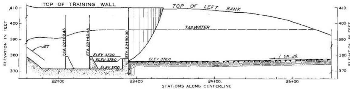
WATER-SURFACE PROFILE
