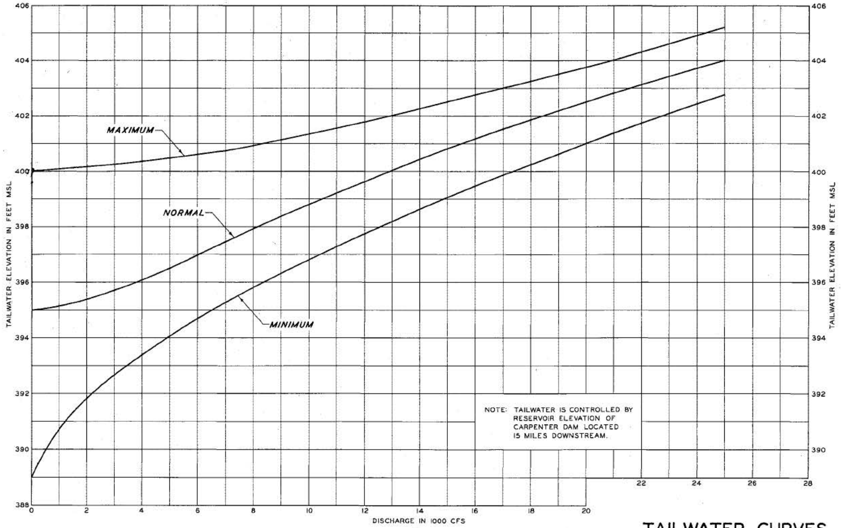
TAILWATER CURVES
