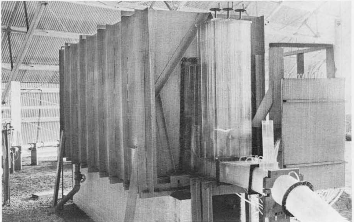
Fig. 3. View of intake tower installed in headbay
