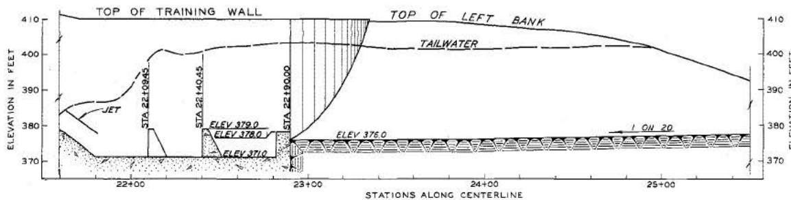
WATER-SURFACE PROFILE
