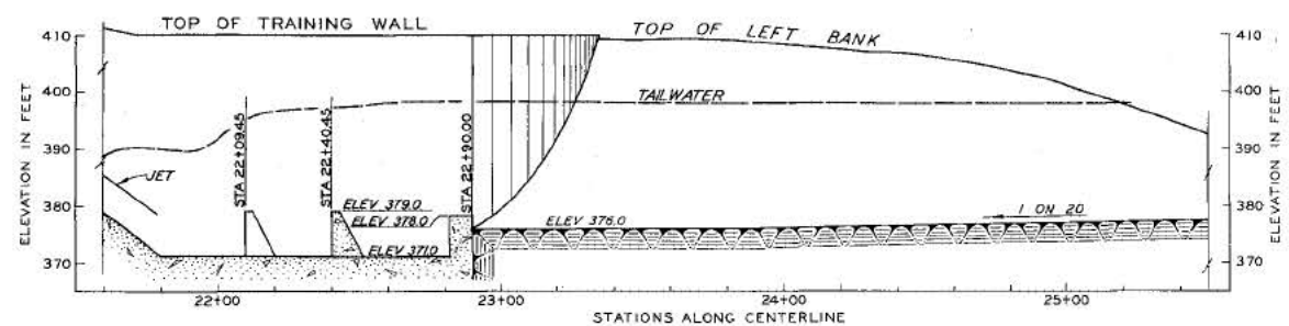
WATER-SURFACE PROFILE
