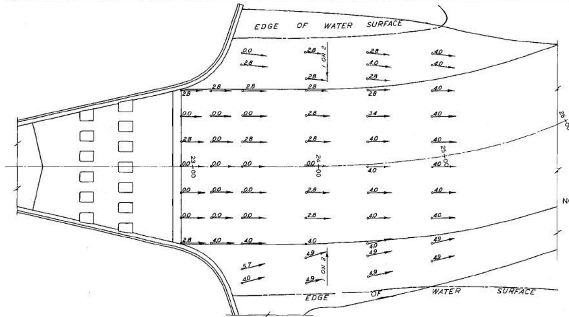
VELOCITY DISTRIBUTION
