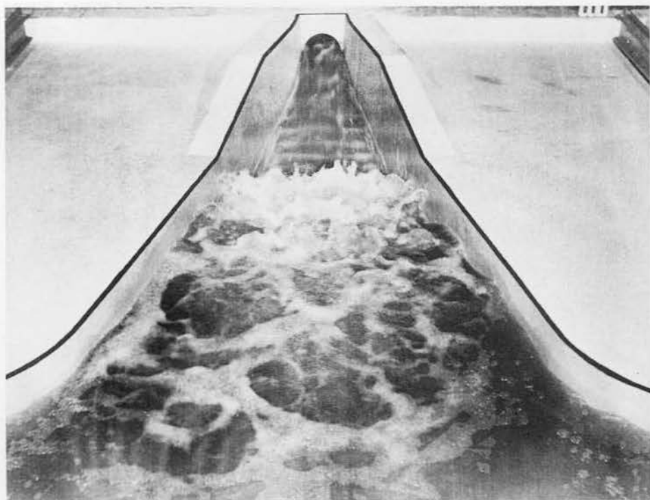
Photograph 10. Discharge, 15,000 cfs; pool elev, 580.0; TW elev, 399.0 Stepped transition, note air pockets on steps
