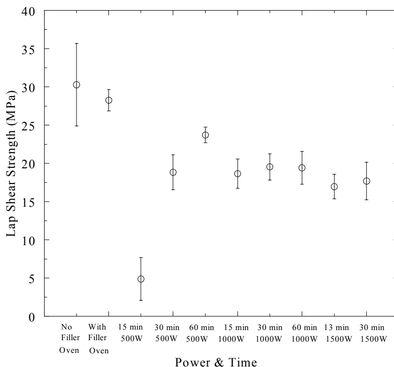
Figure 123. Average lap shear strengths for all processing conditions.
