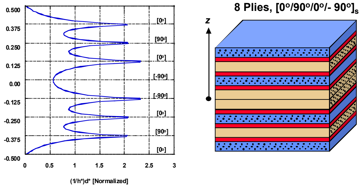
Figure 141. Model Through-Thickness Heat Generation of an 8-Ply Carbon-Fiber Laminate With Orientation [0/90/0/-90]_s
