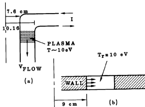
Figure 1. a) Sketch of experimental configuration, b) sketch 1D calculation.
