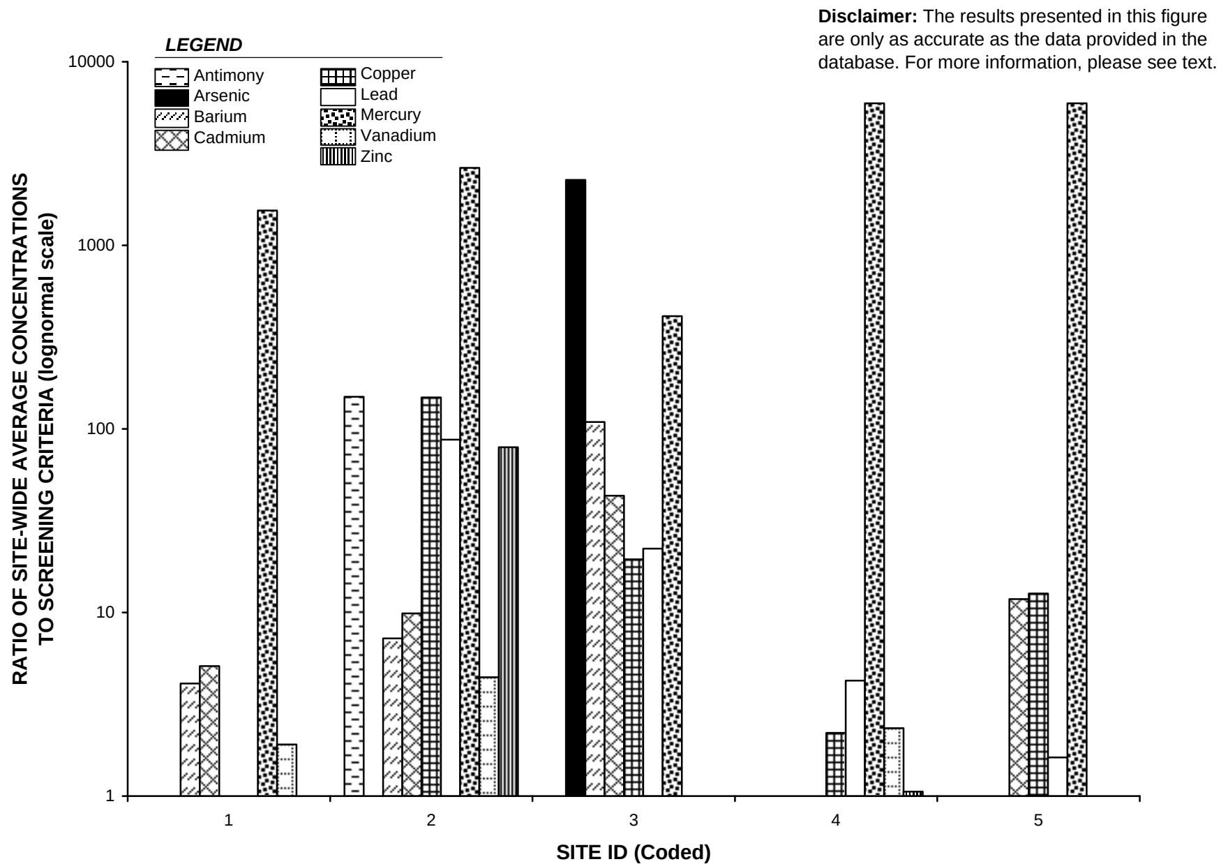
Figure 7c. Ratio of site-wide average concentrations to Mammalian Screening Criteria for the five sites with the highest total risk across all metals. Source: Navy data set.
