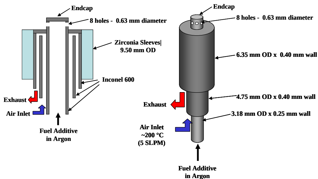
Figure 7 Diluter used in the PFR section of NIST WSR/PFR.
