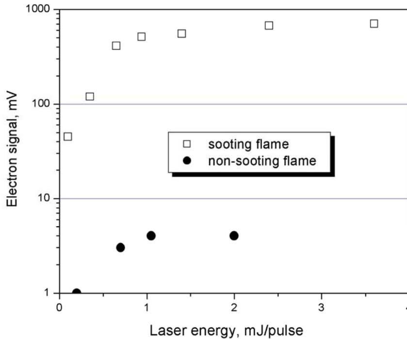
Figure 1 Electron signal (the first peak) as a function of laser energy for both sooting ( \phi = 2.7 ) and non-sooting ( \phi = 2.3 ) flame stoichiometry. Single electrode configuration.
