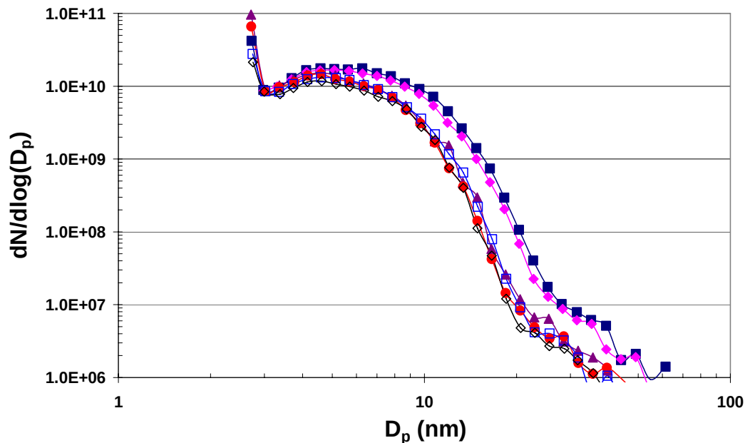
Figure 8 Soot size size distribution in the WSR section of the WSR/PFR at different cross section radii for ethylene/air ( \Phi = 2.0 , 175 SLPM air) using the coannular dilution probe: (■) WSR surface, Scan #1; (◆) WSR surface, Scan #2; (▲) WSR half radius, Scan #1; (●) WSR half radius, Scan #2; (□) WSR centerline, Scan #1; (◇) WSR centerline, Scan #2.
