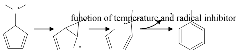
Scheme V. Ring expansion of isopropyl-5-Cp radical.
