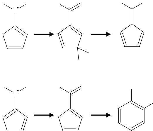
Scheme VI. Alkene formation and subsequent rearrangement from isopropyl-1Cp and isopropyl-2Cp radicals.
