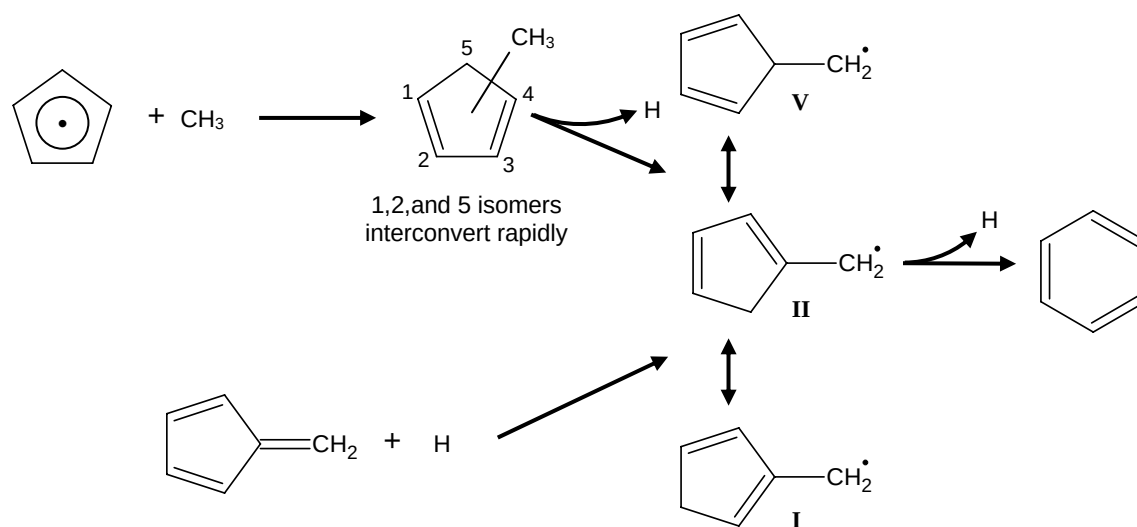
Figure 1. Ring expansion reactions of cyclopentadienyl systems.
