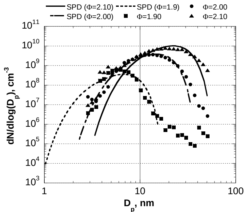
Figure 6 Comparison to self preserving size distribution at free molecular regime for three equivalence ratios.
