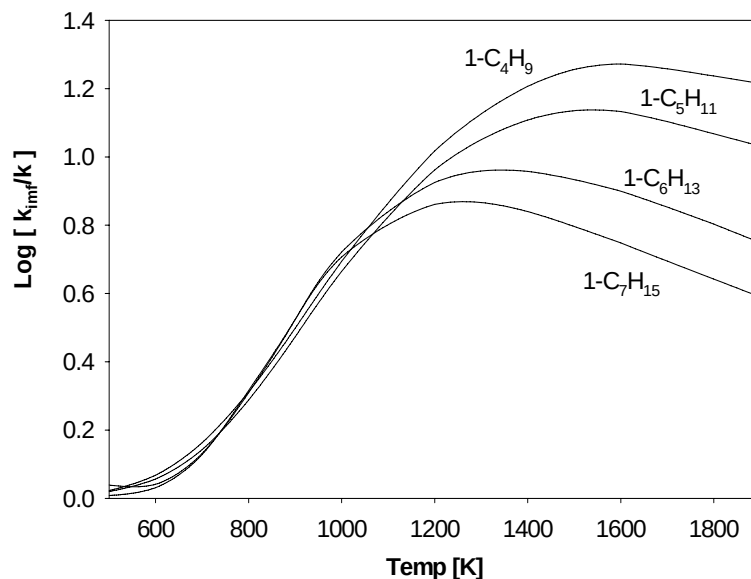
Figure 12: Departure from high pressure behavior for the beta bond scission reactions of various 1-alkyl radicals,
