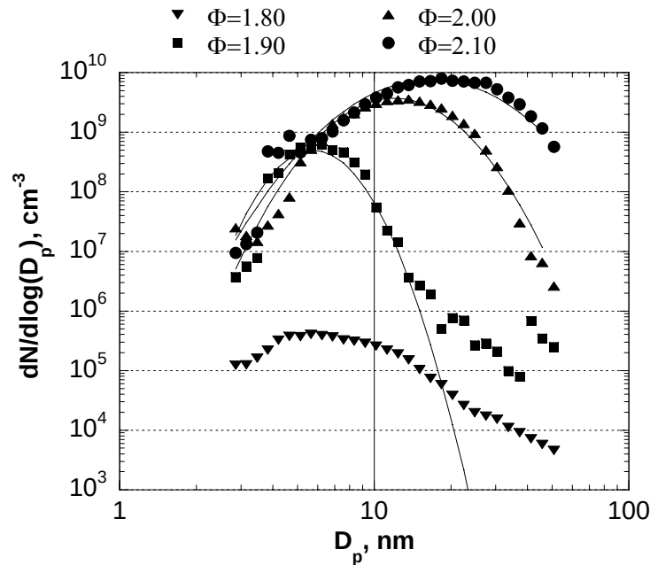
Fig.1 Soot size distributions obtained with the Nano-DMA are plotted for the WSR operating at four equivalence ratios close to the point of soot inception. At \Phi = 1.8 , there was no indication of flame generated particles. Lognormal fits are applied to the distributions.
