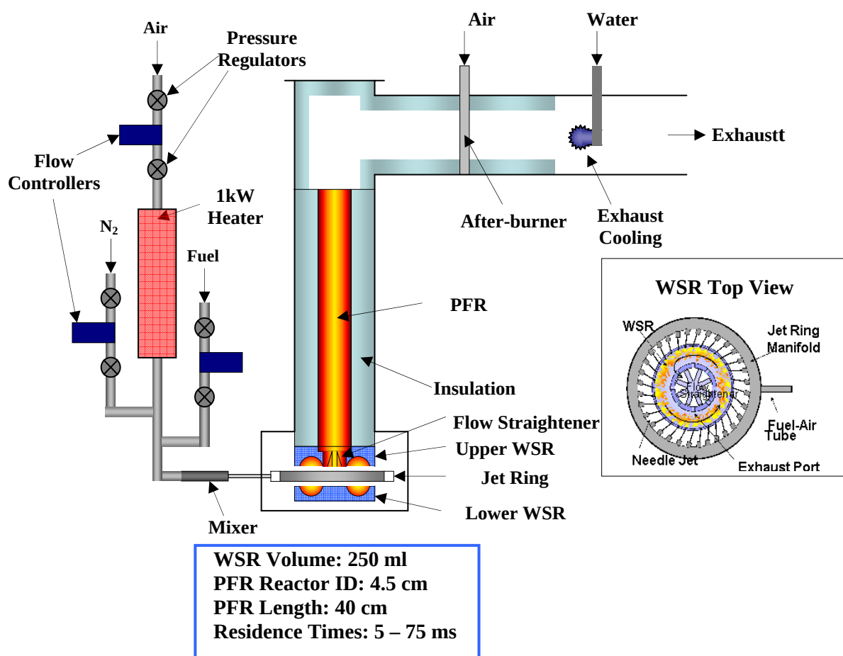
Figure 1 NIST Well Stirred Reactor/Plug Flow Reactor (WSR/PFR)
