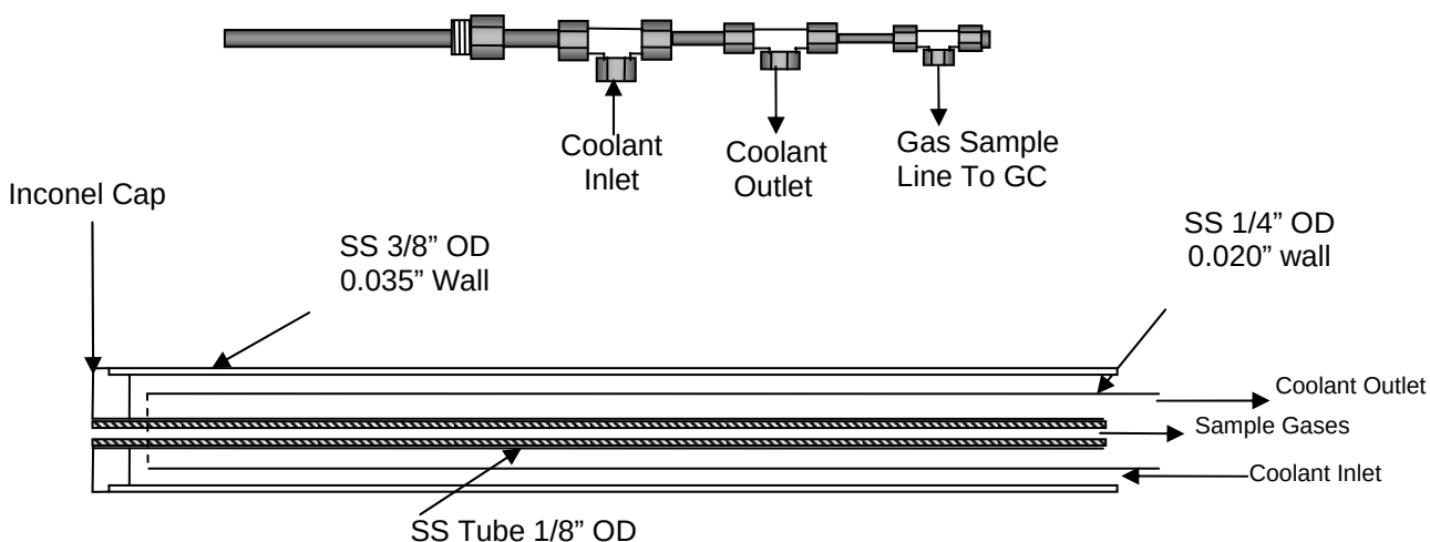
Figure 1 Schematic of oil cooled gas sampling probe
