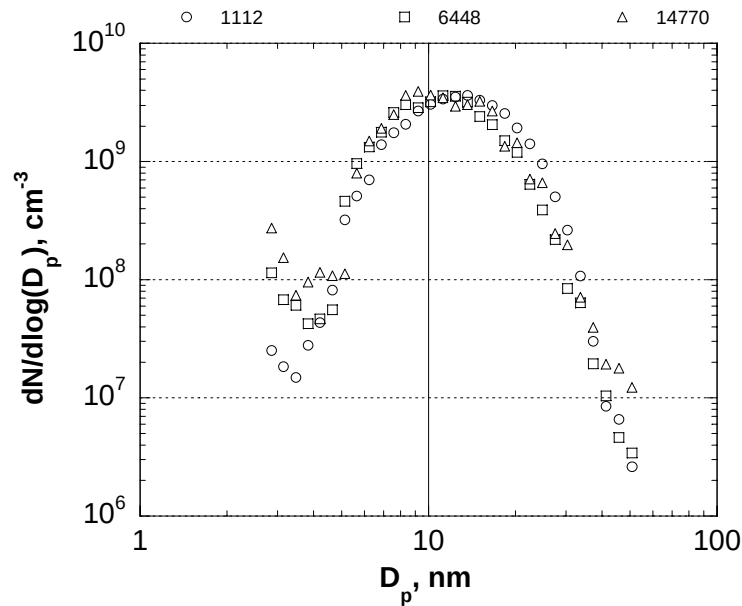
Figure 2 The effect of the dilution ratio on the measured soot size distribution. Experimental conditions: equivalence ratio, \Phi = 2.0 , dilution ratio varied from 1112 to 14770.
