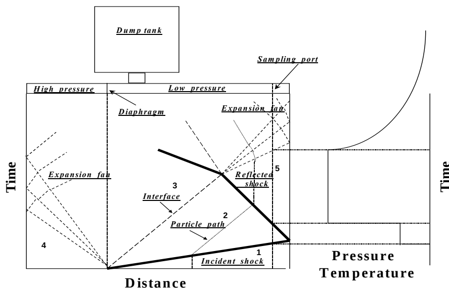
Figure 5: Schematic of single pulse shock tube and associated wave diagrams.
