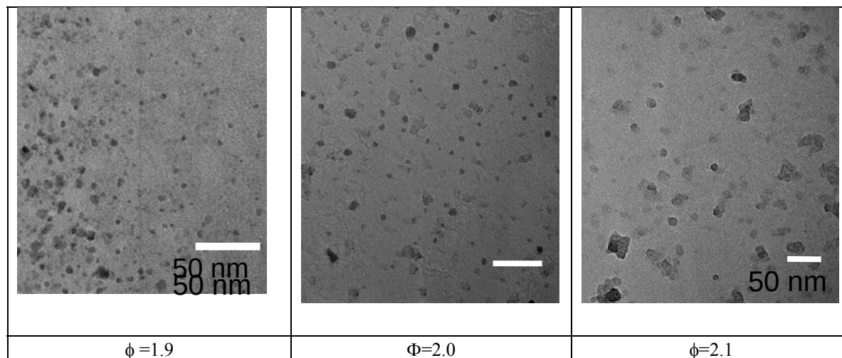
Figure 5 TEM Images of Soot Particles Collect for Ethylene/Air Combustion
