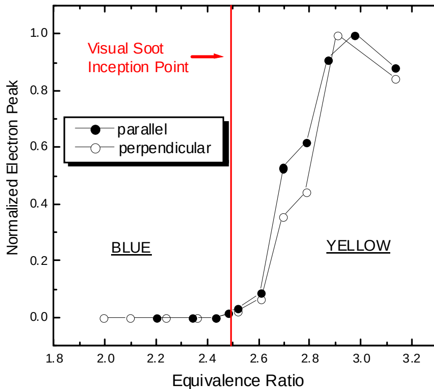
Figure 5 The variation of normalized electron signal intensity as a function of equivalence ratio for parallel and perpendicular electrode configurations. Electrode biased at -700 V.
