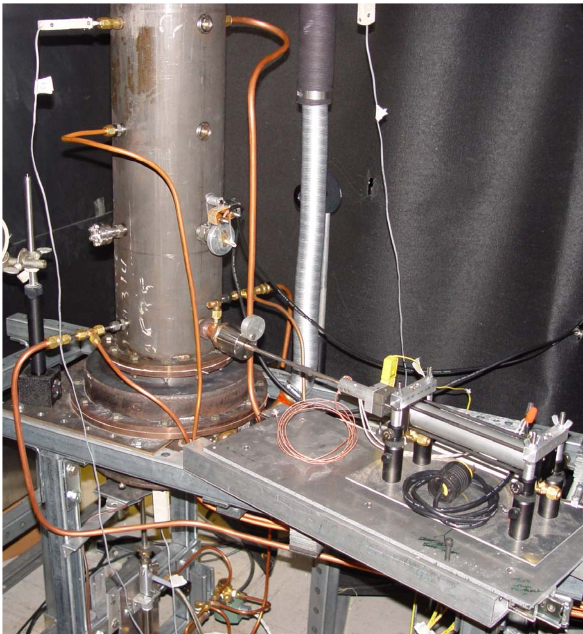
Figure 4 Picture of the TEM sampling probe. The PFR section is shown.
