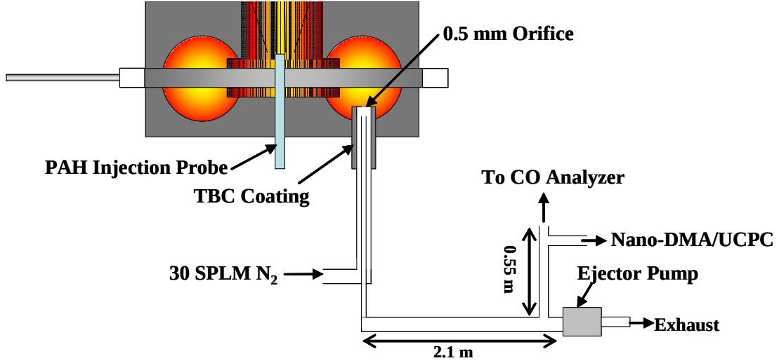
Figure 6 Diluter used in the PFR section of NIST WSR/PFR.
