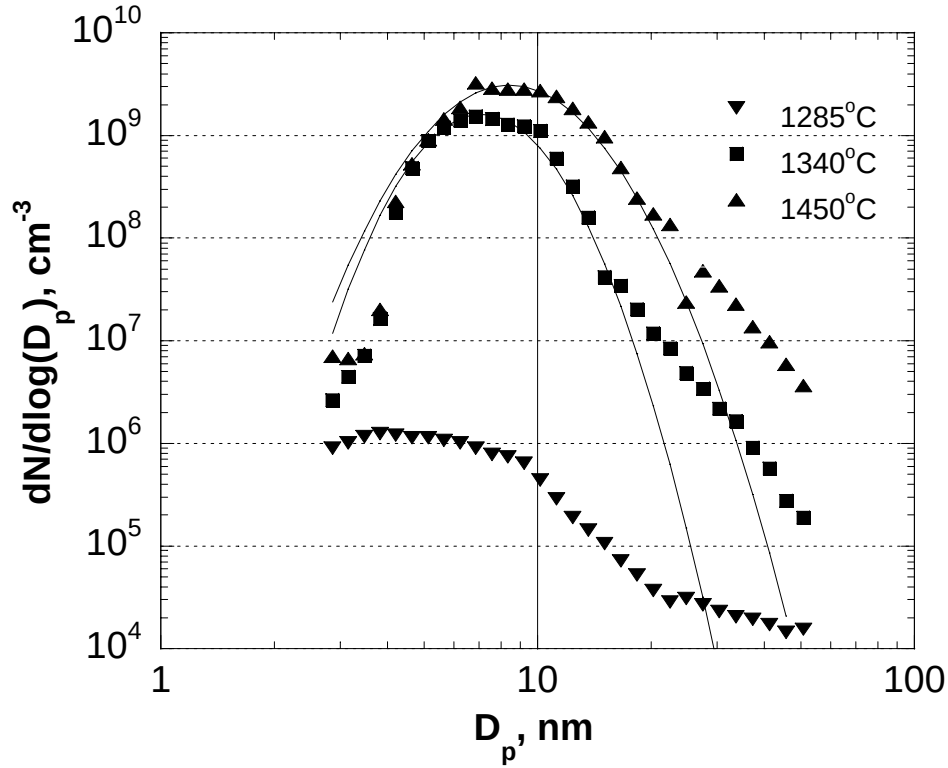
Figure 3 The effect of temperature on the measured soot size distribution. Experimental conditions: dilution ratio 1000, equivalence ratio, \Phi = 2.0 . Lognormal fits are applied to the distributions.
