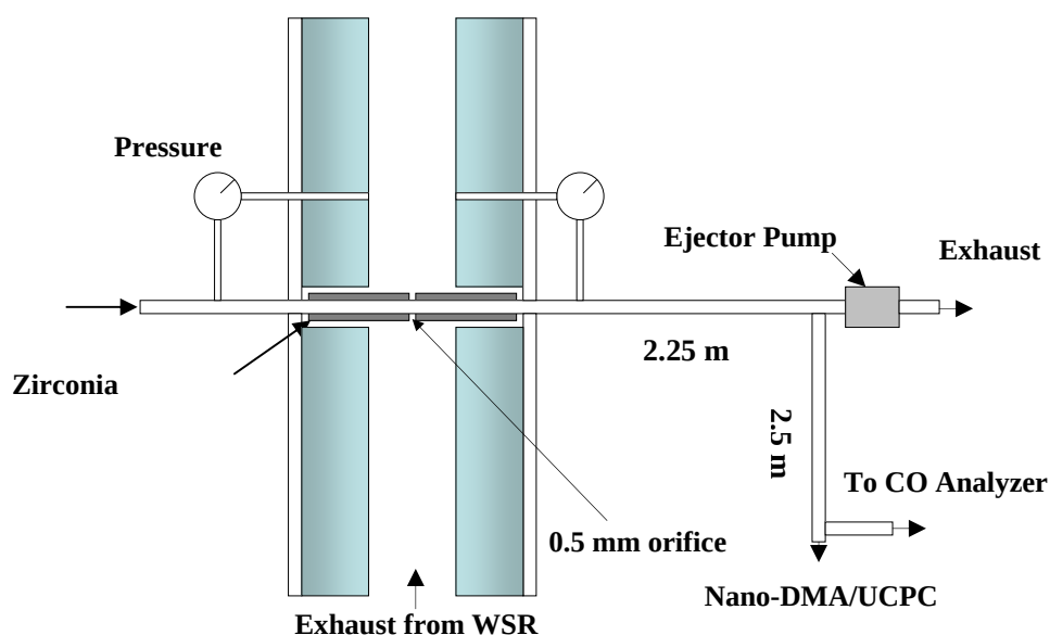
Figure 5 Diluter used in the PFR section of NIST WSR/PFR.
