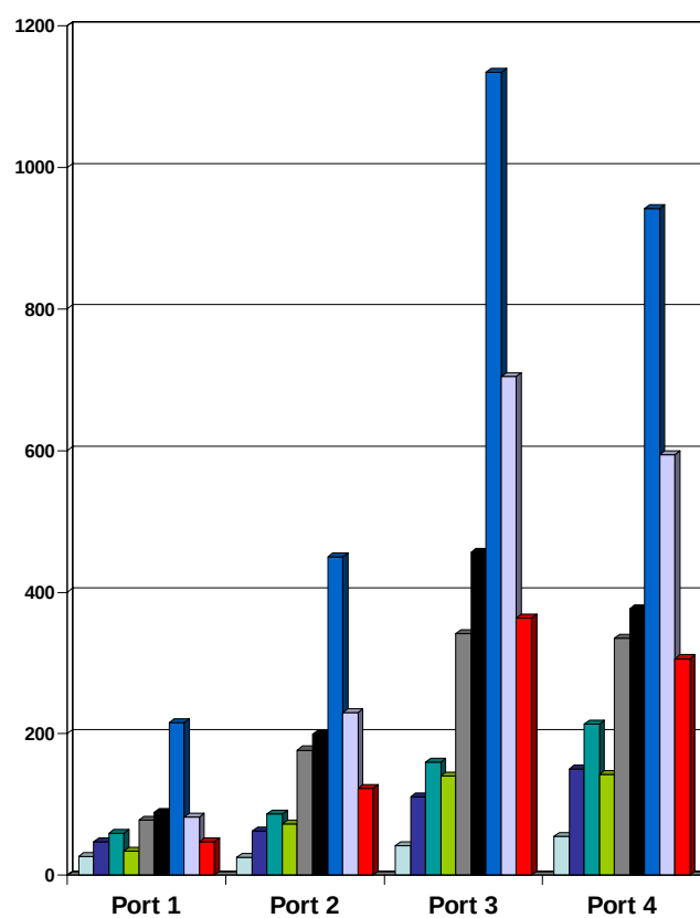
Figure 6 Selected PAHs on Top Filters-Benzene Addition
