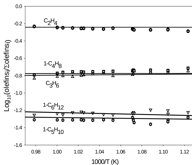
Figure 6: Branching ratio for olefin production during the decomposition of heptyl-1 [4]
