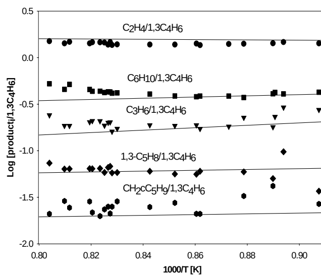
Figure 7 Branching ratios in terms of olefin to 1,3-butadiene during the decomposition of cyclohexyl radicals from tertbutyl cyclohexane
