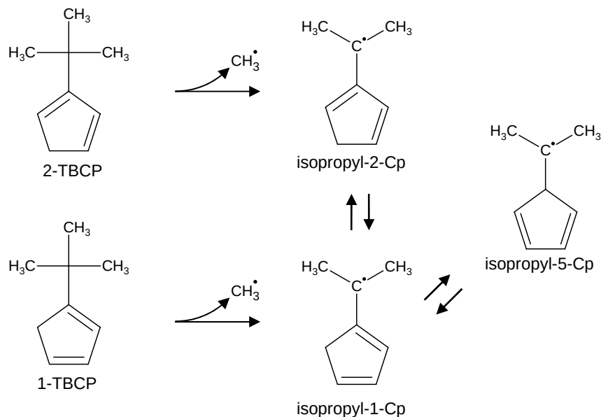
Scheme IV. \text{CH}_3 -loss channels and subsequent isomerization of 1-TBCP and 2-TBCP.
