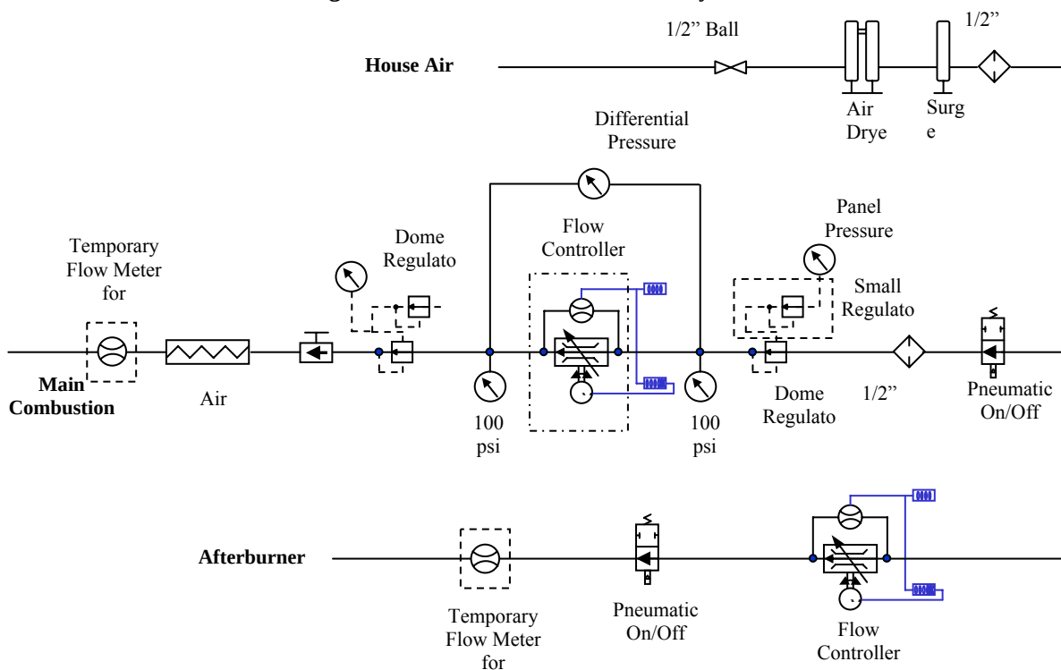
Figure 3 NIST WSR/PFR Air Flow System
