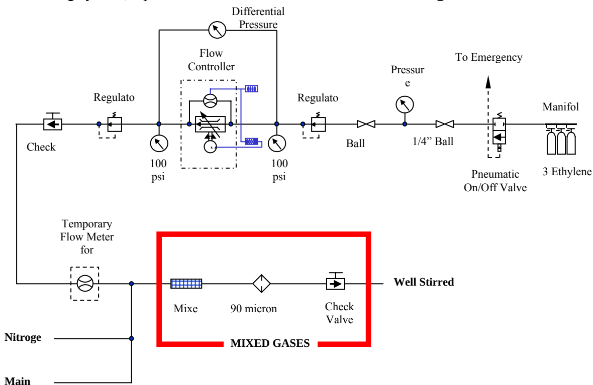
Figure 2 NIST WSR/PFR Main Fuel System
