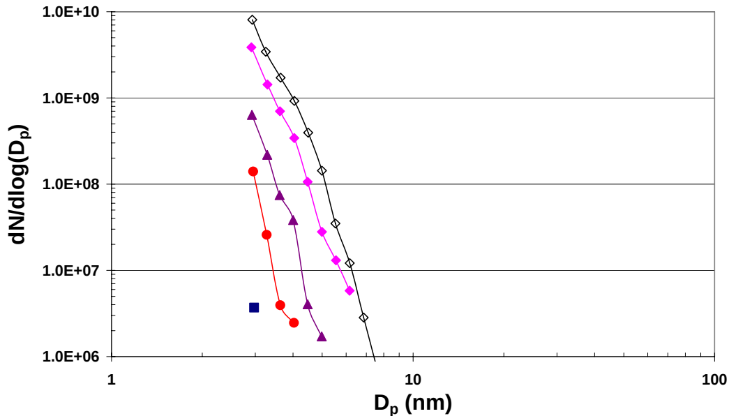
Figure 10 Soot size size distribution using the linear probe in the PFR section of the WSR/PFR for ethylene/air/nitrogen with naphthalene/methanol injection ( \Phi = 1.8 , 175 SLPM air, 30 SLPM nitrogen): (■) 1.90 ml/min Methanol injection, Port #3; (●) 0.96 ml/min Naphthalene/Methanol injection, Port #3; (▲) 1.41 ml/min Naphthalene/Methanol injection, Port #3; (◆) 1.90 ml/min Naphthalene/Methanol injection, Port #3; (◇) 2.47 ml/min Naphthalene/Methanol injection, Port #3.
