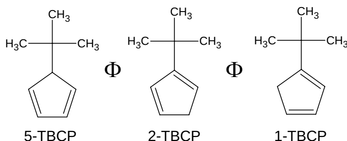
Scheme I. Isomerization of t -butyl cyclopentadiene.
