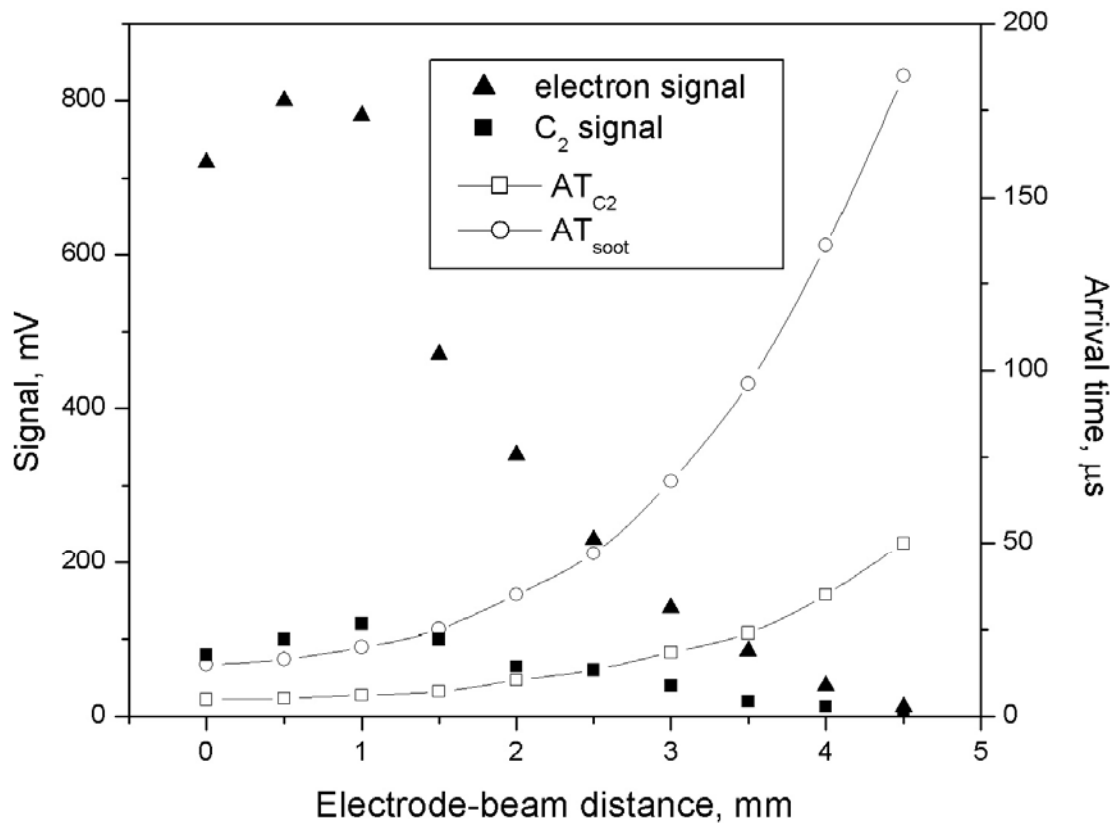
Figure 4 The effect of electrode laser-beam distance on the peak amplitude and arrival time of ions. The experimental conditions: \phi = 2.69 , laser energy = 0.6mJ/pulse, electrode biased at -500V, laser beam 1 cm above burner head.
