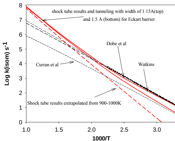
Figure 10: Rate constants for 1-5 H-transfer isomerization for 1-hexyl radical[12-14]
