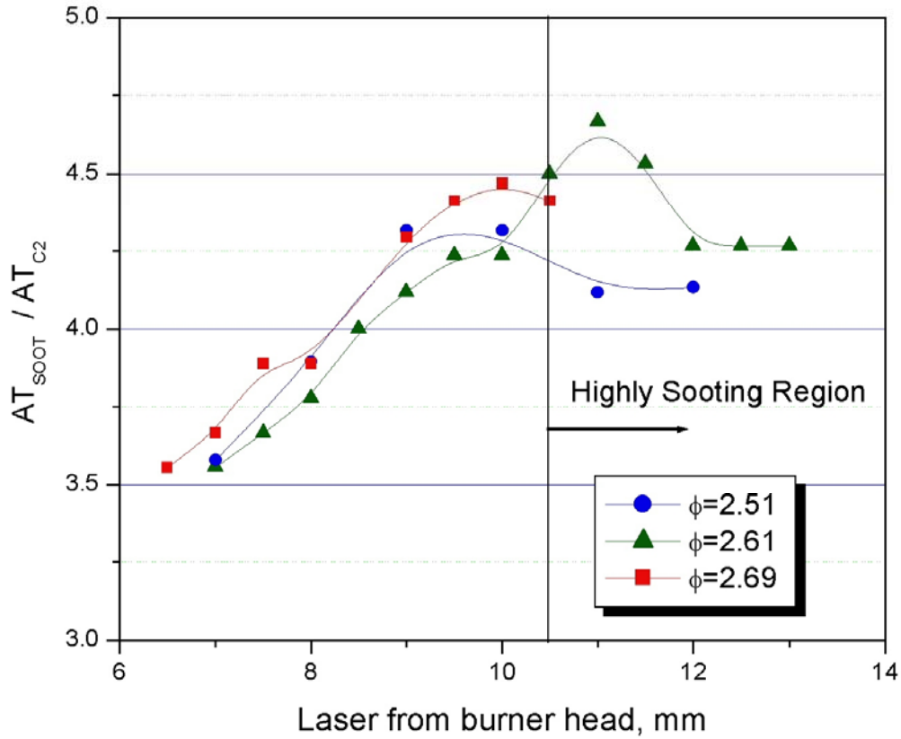
Figure 2 The ratio of soot ion arrival time to C_2^+ ion arrival time as a function of laser beam to burner head distance for three different equivalence ratios. The electrode-laser beam distance was fixed. The data were obtained using the single electrode configuration with the electrode biased at -700 V.
