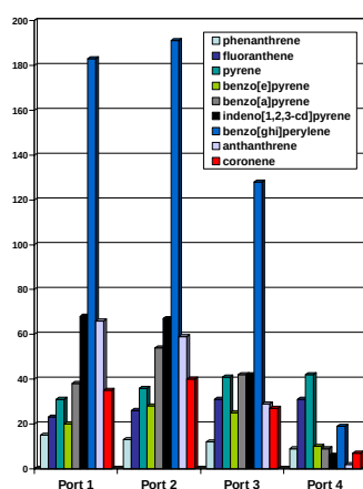
Figure 4 Selected PAHs on Top Filters-No Benzene
