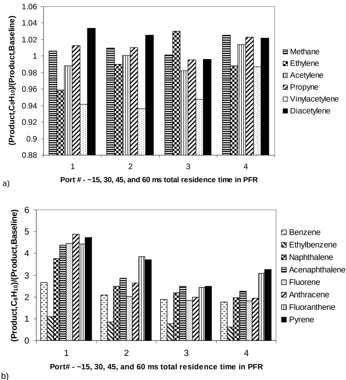
Figure 3 Comparison of changes in gas phase species concentration as a function of increasing residence time with the addition of 526 ppm of ethylbenzene at ~1300 K and 1 bar. a) lighter hydrocarbons (less than C 6 ) b) heavier hydrocarbons (C 6 or greater)
