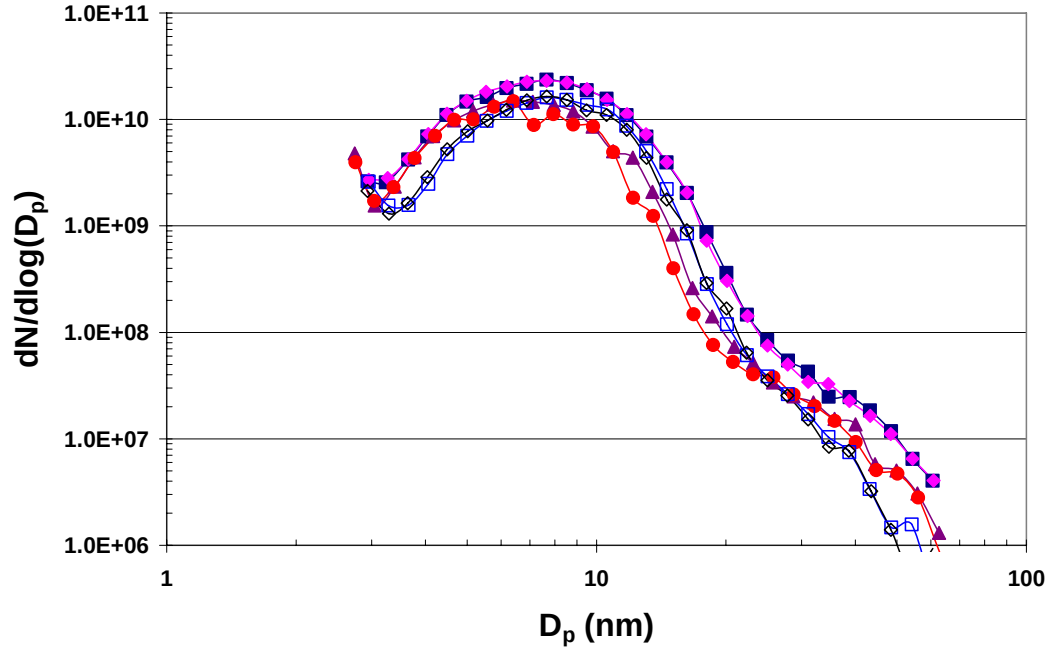
Figure 7 Soot particle size distribution in the PFR section of the WSR/PFR at two different residence times and two different probe designs for ethylene/air ( \Phi = 2.0 , 175 SLPM air): (■) Linear probe, Port #1, Scan #1; (◆) Linear probe, Port #1, Scan #2; (▲) Coannular probe, Port #1, Scan #1; (●) Coannular probe, Port #1, Scan #2; (□) Linear probe, Port #3, Scan #1; (◇) Linear probe, Port #3, Scan #2.
