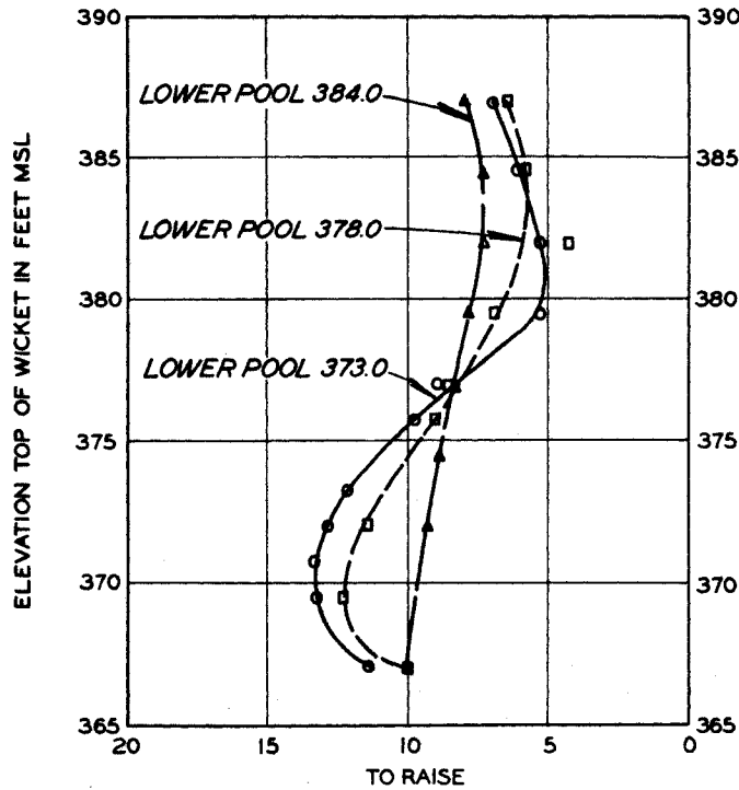
FORCE IN 1,000 POUNDS
