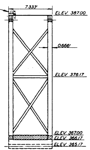
DOWNSTREAM ELEVATION WICKET RAISED
