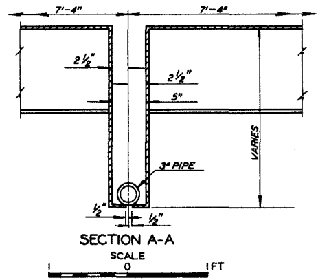
CURVED WICKET REVISED DESIGN
