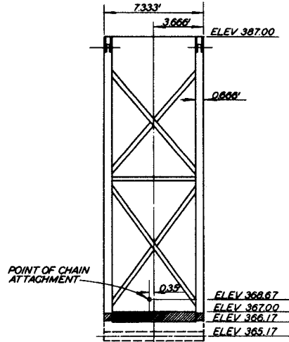
DOWNSTREAM ELEVATION WICKET RAISED
