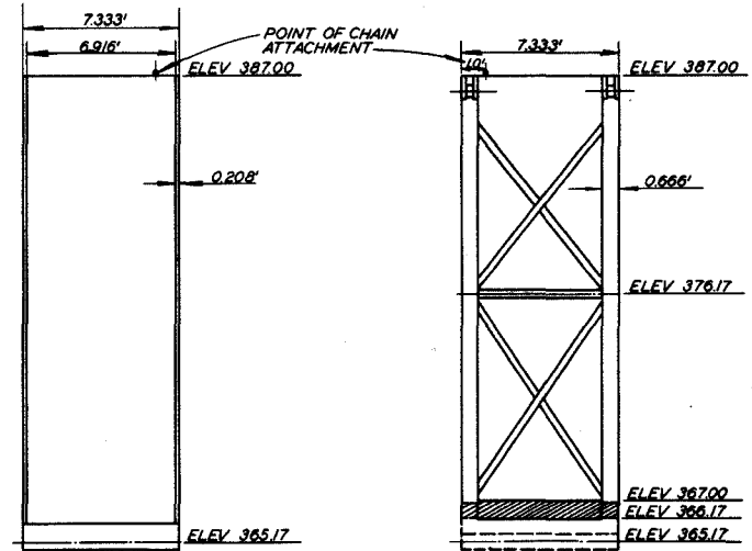
UPSTREAM ELEVATION WICKET RAISED DOWNSTREAM ELEVATION WICKET RAISED
