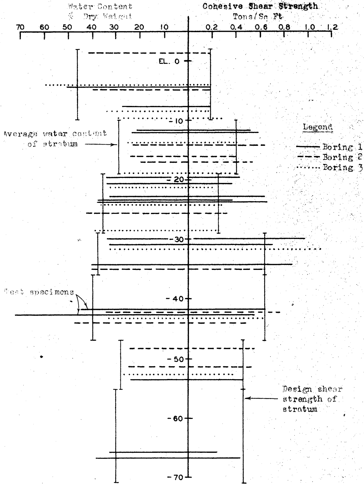
Waterways Experiment Station Catfish Point Control Structure WATER CONTENTS AND COHESIVE SHEAR STRENGTH Borings 1, 2, and 3 November 1947 Plate 3095-17
