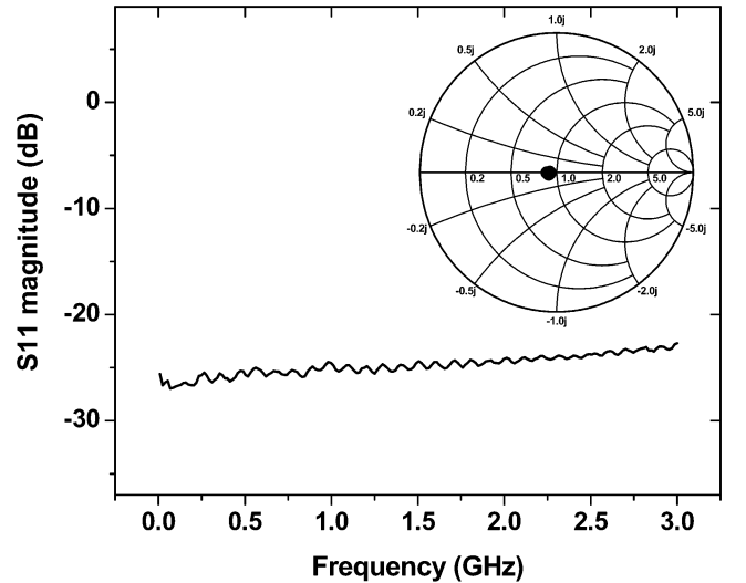
Fig. 6. S_{11} reflection coefficient of the 45 \Omega resistive actuator.
